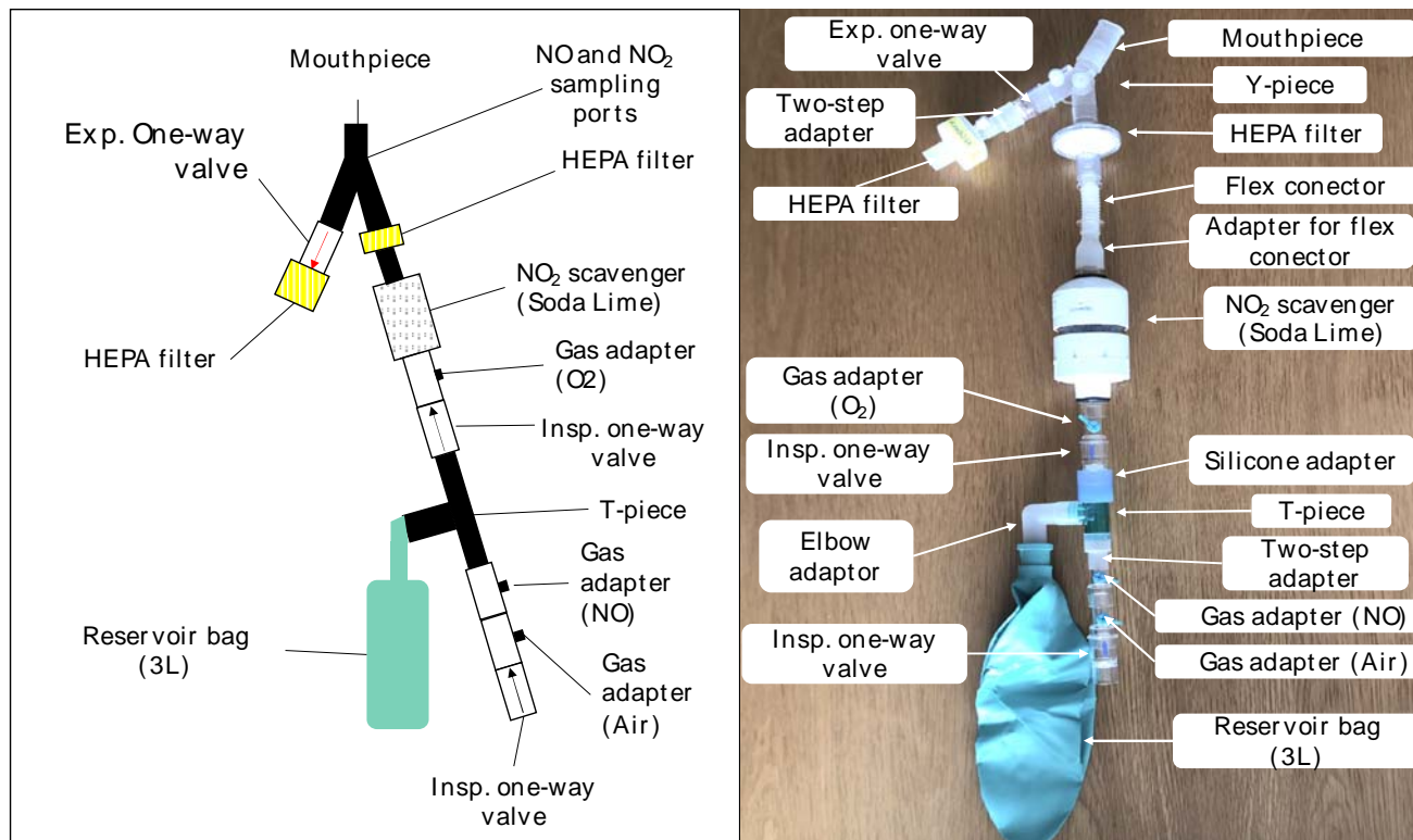
Figure 2. Nitric oxide gas delivery system.
