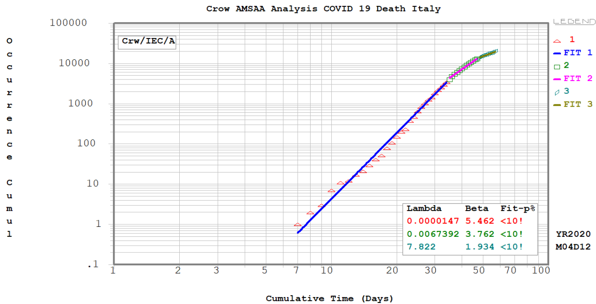
Fig 12. The piece wise Crow-AMSAA analysis for COVID 19 Deaths –Italy
