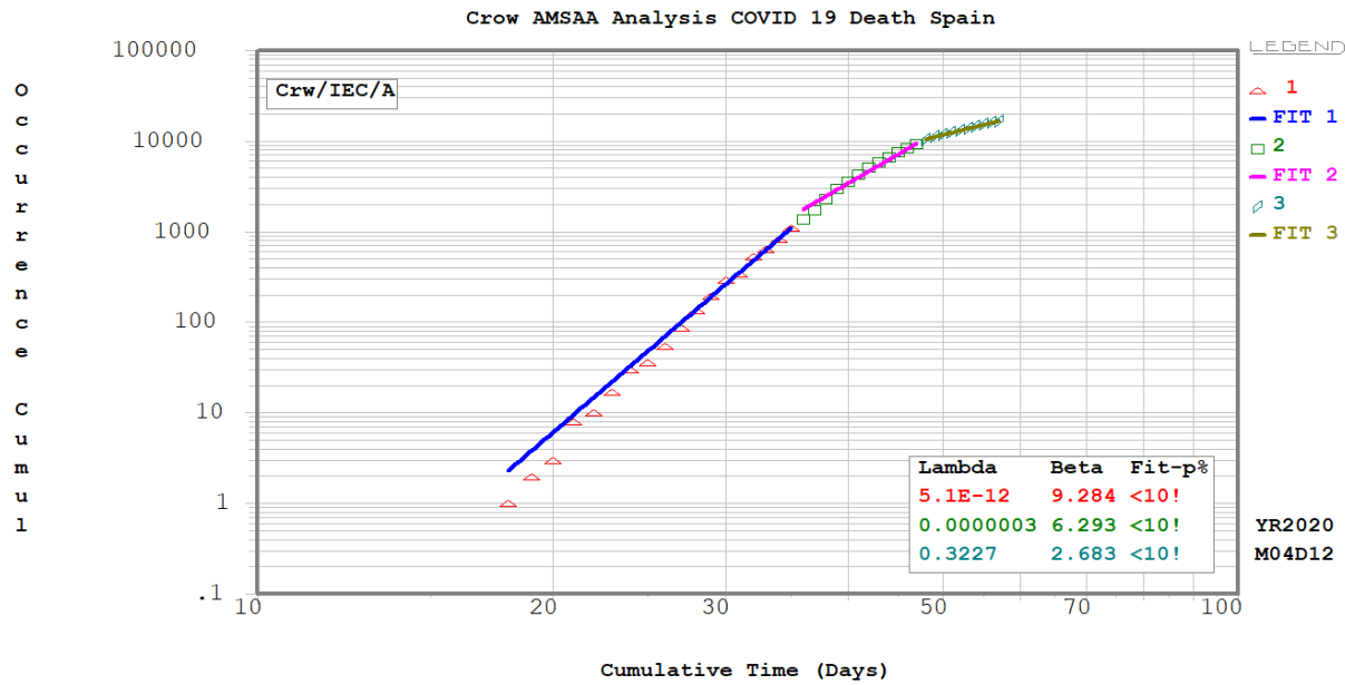
Fig 10. The piece wise Crow-AMSAA analysis for COVID 19 Deaths –Spain
