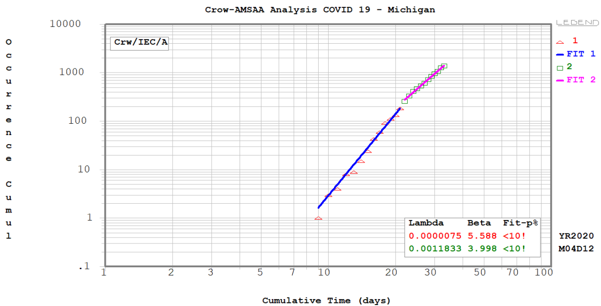
5 Fig 6. The piece wise Crow-AMSAA analysis for COVID 19 Deaths –Michigan
