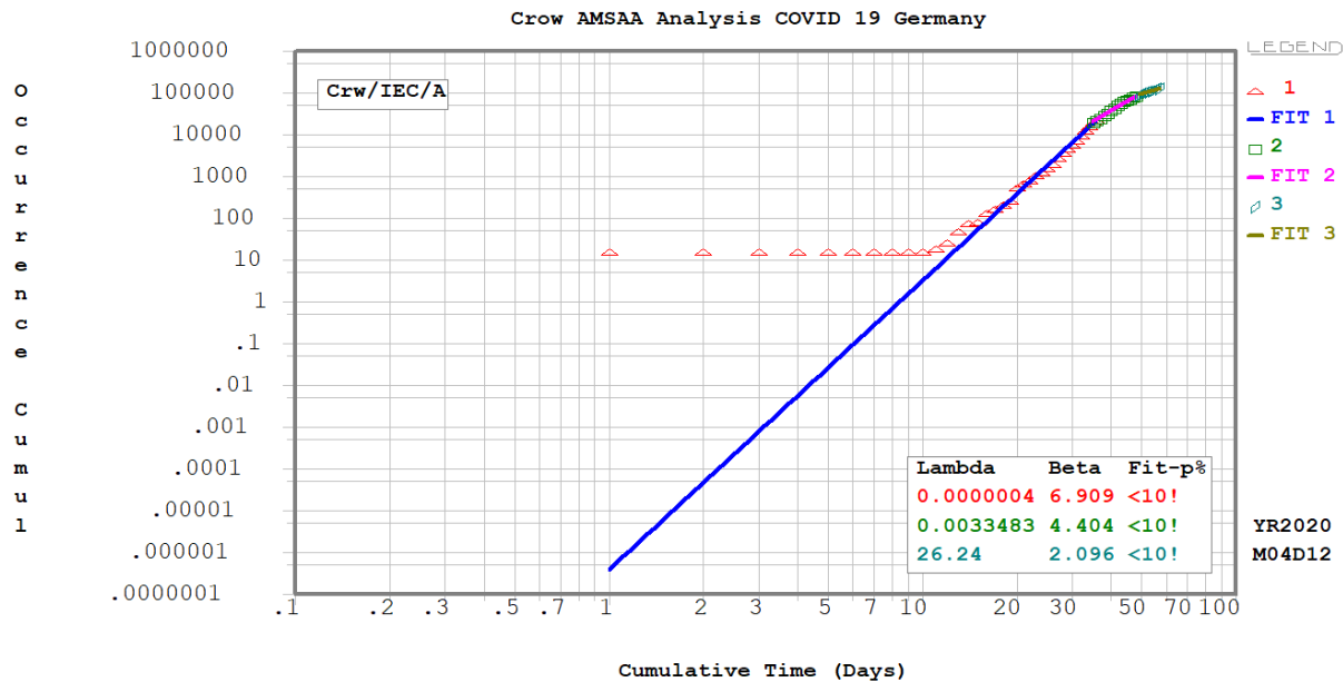
Fig 20. The piece wise Crow-AMSAA analysis for COVID 19 –Germany
