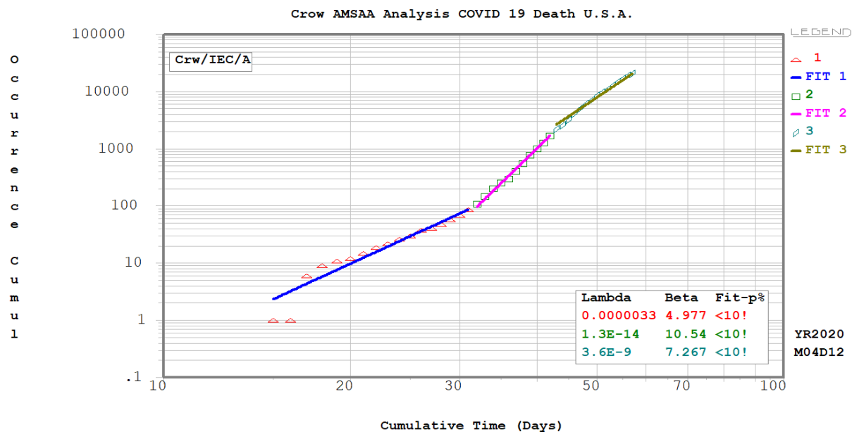
5 Fig 8. The piece wise Crow-AMSAA analysis for COVID 19 Deaths –U.S.A
