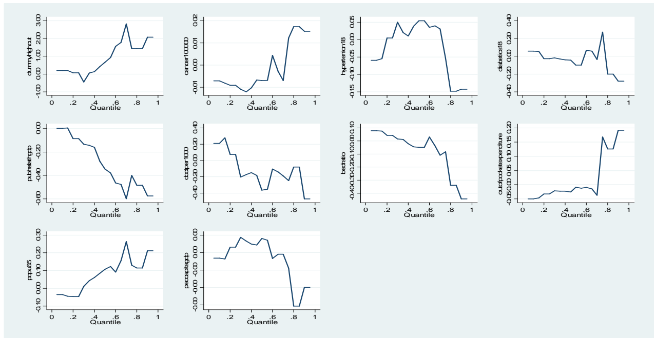
Figure 2: The coefficients of a Quantile Regression (Model-1)
