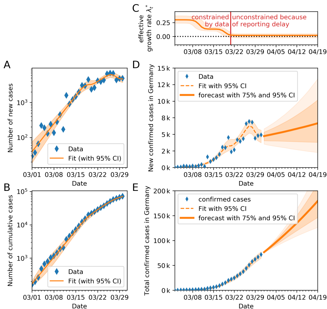
FIG. 3. The data until March 31 indicates two change points, consistent with the first two governmental interventions. Assuming a model with two change points, we infer the spreading rates \lambda_i from the observed COVID-19 case numbers in Germany (blue dots). We then forecast the future development of case numbers (orange line), assuming no further change points here. For the same approach with one or three change points, please see the corresponding figures in the SI (Fig. S1 and S3). Prior and posterior distributions of all model parameters are reported in Fig. 4. A : Comparison of daily recorded new cases and the model, log scale. B : Comparison of total recorded cases and the model, log scale. C : Time-dependent model-estimate of the effective spreading rate \lambda_t^* . D : Model forecast of new cases, based on the inferred \lambda_t , linear scale. E : Model forecast of total cases, based on the inferred \lambda_t , linear scale.
