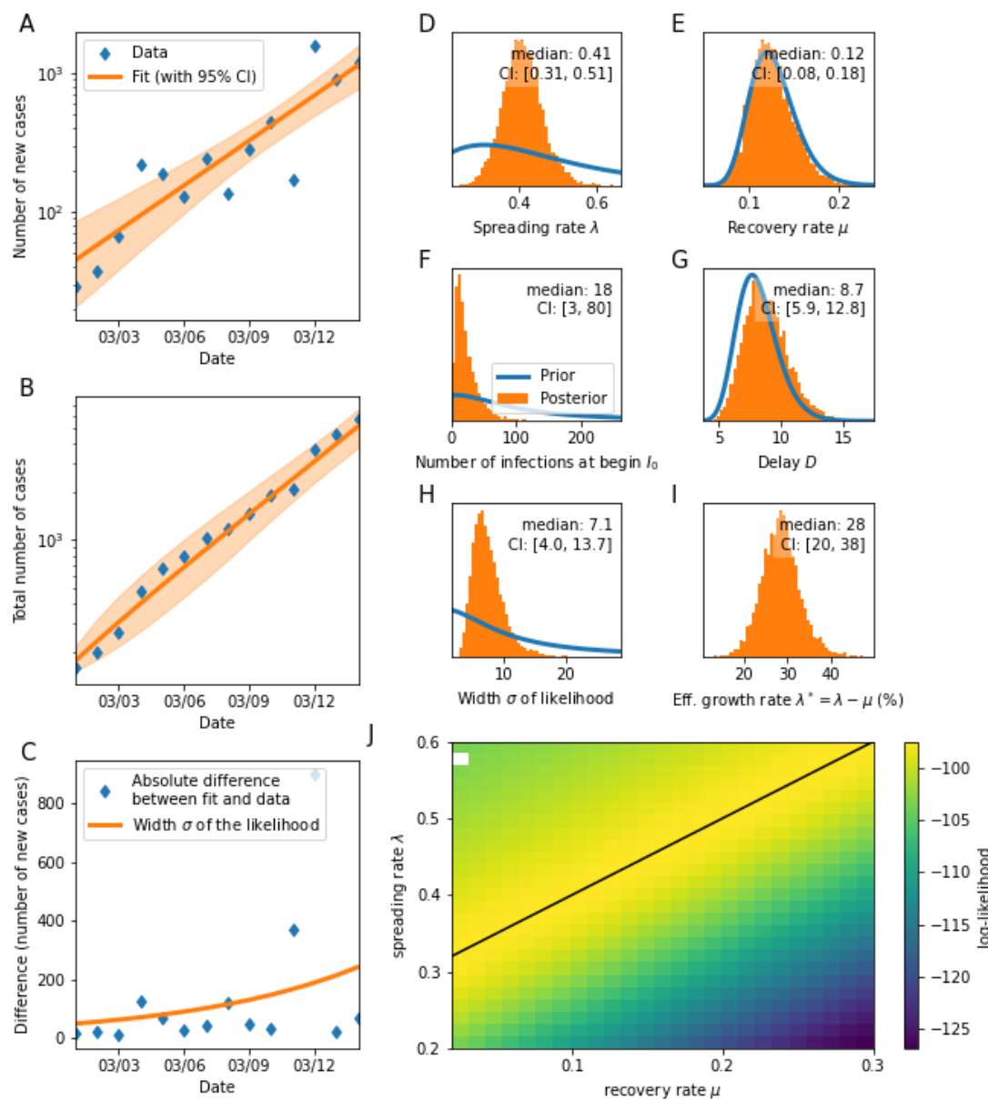
FIG. 1. Central epidemiological parameters of the SIR model are constrained by the initial onset period (March 1st–15th). A : Number of new cases over time. B : Same as A but for total number of cases over time (cumulative). C : Absolute difference between model and data (blue line) is captured by the demographic-noise width scale-factor \sigma we chose for the likelihood (Student's t-distribution). The error of the likelihood function scales with the number of new cases as \sigma\sqrt{C_t} . D-I : Prior (blue) and posterior (orange) distributions for all model parameters: estimated spreading rate \lambda , recovery rate \mu , reporting delay D between infection date and reporting date, number of cases I_0 at the start of the simulation, width scale-factor \sigma of the likelihood distribution and the effective growth rate \lambda^* = \lambda - \mu (calculated from \lambda and \mu ). J : Log-likelihood distribution for different combinations of \lambda and \mu . A linear combination of \lambda and \mu yield the same maximal likelihood (black line).
