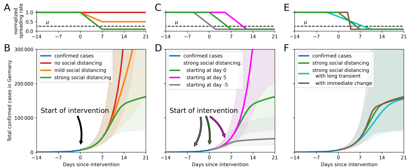
FIG. 2. The timing and effectiveness of interventions strongly impact future COVID-19 cases in Germany. A, B: We assume three differently scenarios for interventions starting on 2020/03/15: (I) no social distancing — red, (II) mild social distancing — orange, or (III) strict social distancing — green. C, D: We also analyzed how a delayed restriction impacts case numbers: Strict restrictions starting on 2020/03/15 (green), or five days later or earlier. A delay (or advance) of five days in implementing restrictions has a major impact on the expected case numbers. E, F: Comparison of the time span over which interventions ramp up to full effect. For all ramps that are centered around the same day , the resulting case numbers are fairly similar.
