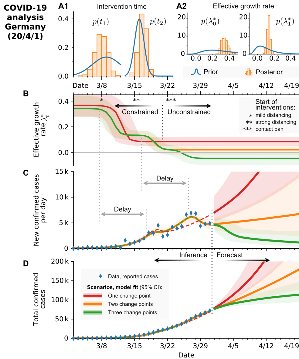
FIG. 1. [This figure uses data available as of April 1st. On our github repository you find the current figure versions.] Inference of spreading rate \lambda from confirmed COVID-19 cases in Germany, and forecast of future evolution. A: Prior (blue) and posterior (orange) distributions for four of the central parameters of a SIR model with two change points (at time t_1 and t_2 ), where the spreading rate changes from \lambda_0 \rightarrow \lambda_1 \rightarrow \lambda_2 . B: The inferred effective growth rate \lambda^* , i.e. the difference between spreading and recovery rate ( \lambda^* = \lambda - \mu ) for an SIR model which assumes one, two or three change points (red, orange, green). The models with two or three change points are favored over the one with one change point by formal Bayesian model comparison. The inferred change points correspond well to the timing of the governmental interventions in Germany (depicted as *). C,D: The model fit of the new confirmed cases and (cumulative) total confirmed cases is depicted for the models with one, two or three change points. The three future scenarios depend strongly on whether one includes the second or third change point: the number of new confirmed cases will grow exponentially, be approximately constant, or decay exponentially (red, orange, green). Hence, the future development depends predominantly on our behavior. B,C: Note the delay D between change point (i.e. change in spreading behavior) and observation of confirmed cases of almost two weeks.
