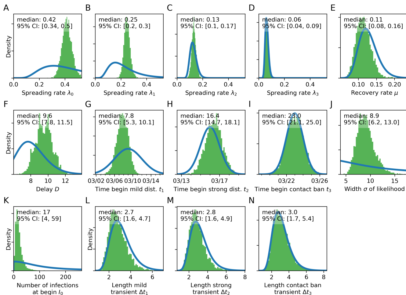
FIG. S4. Posterior distributions from the change-point detection with three change points (green) compared to prior distributions (blue). Please refer to Fig. 4 for a more detailed description of the distributions.
