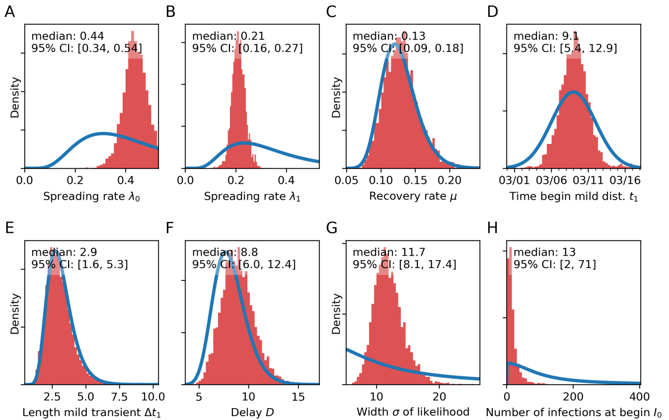
FIG. S2. Posterior distributions from the change-point detection (red) with one change point compared to prior distributions (blue). Please refer to Fig. 4 for a more detailed description of the distributions.
