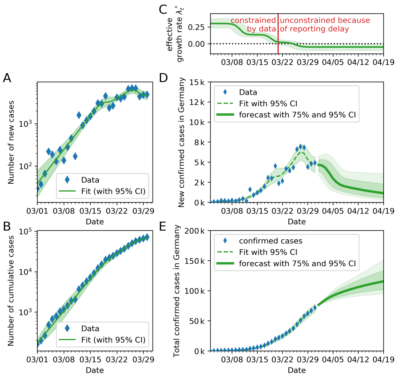
FIG. S3. Inferring and forecasting (the time of) the change point in spreading rate \lambda , assuming three change points. Please refer to Fig. 3 for the case with two change points. A: Comparison of daily recorded new cases and the model, log scale. B: Comparison of total recorded cases and the model, log scale. C: Time-dependent model-estimate of the spreading rate \lambda_t . D: Model forecast of new cases, based on the inferred \lambda_t , linear scale. E: Model forecast of total cases, based on the inferred \lambda_t , linear scale.
