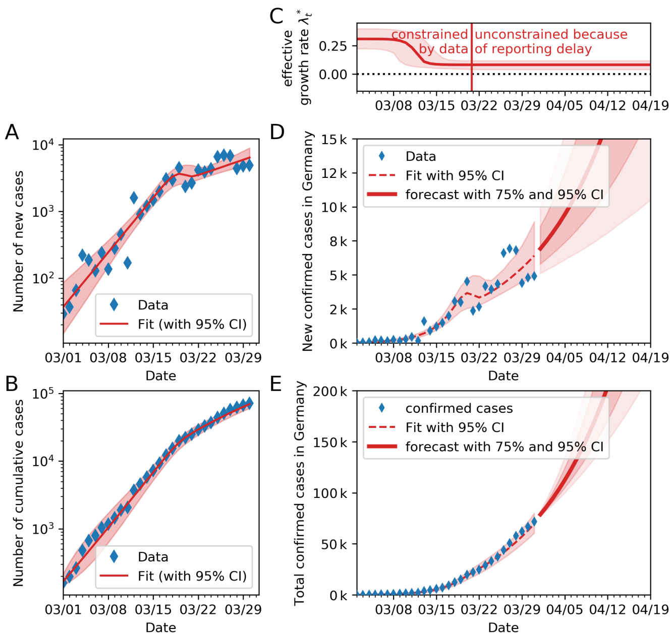
FIG. S1. Inferring (the time of) the change point in spreading rate \lambda , assuming only one change point. Please refer to Fig. 3 for the case with two change points. A: Comparison of daily recorded new cases and the model, log scale. B: Comparison of total recorded cases and the model, log scale. C: Time-dependent model-estimate of the spreading rate \lambda_t . D: Model forecast of new cases, based on the inferred \lambda_t , linear scale. E: Model forecast of total cases, based on the inferred \lambda_t , linear scale.
