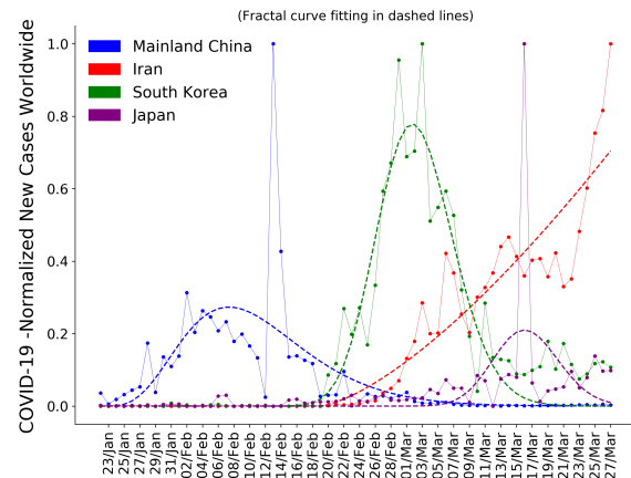
FIG. 1: COVID-19 per country. Illustration of the number of cases and fitting through fractal growth (dashed lines), Eq. (2), for a representative number of countries.
