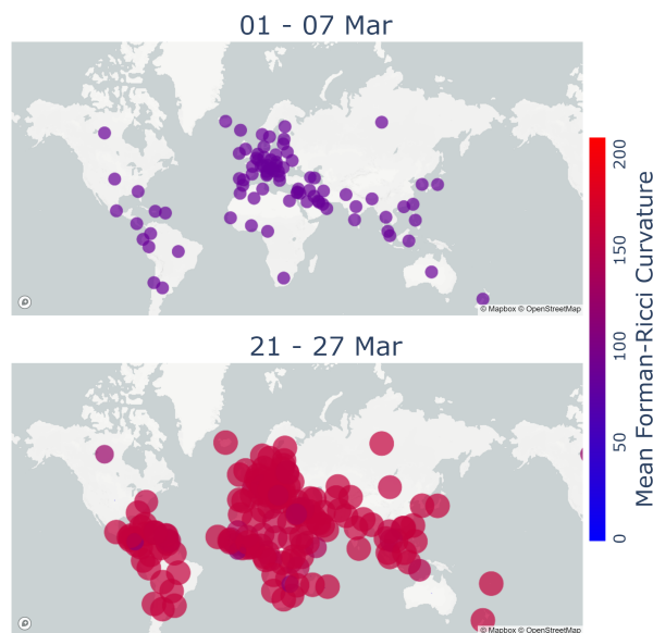
FIG. 5: Illustration of the distribution of the Forman-Ricci curvature for two different time windows based in cumulative cases.
