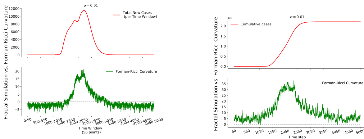
FIG. 3: (Top) Illustration of toy-model epidemic curves, both new cases and cumulative cases, according to (3) and its respective Forman-Ricci curvature at the bottom, with white noise parameter \sigma = 0.01 .
