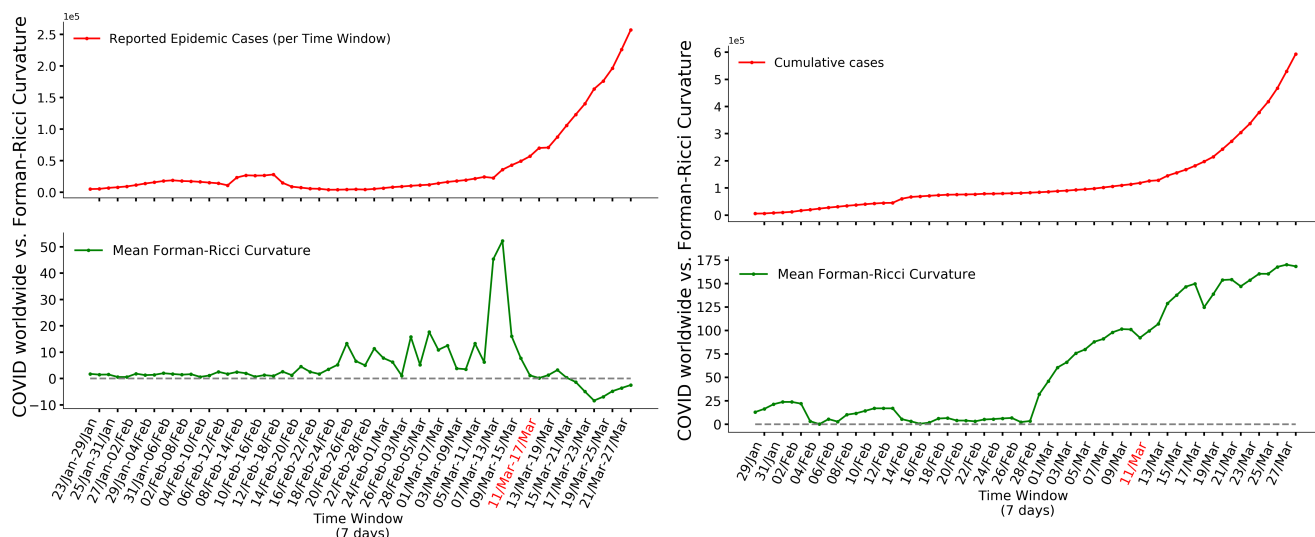
FIG. 4: (Top) Reported epidemic cases per time window, both new cases and cumulative cases, vs. its Forman-Ricci curvature (bottom) for the same time period. In red, we indicate the moment when the WHO declared COVID-19 as a pandemic.
