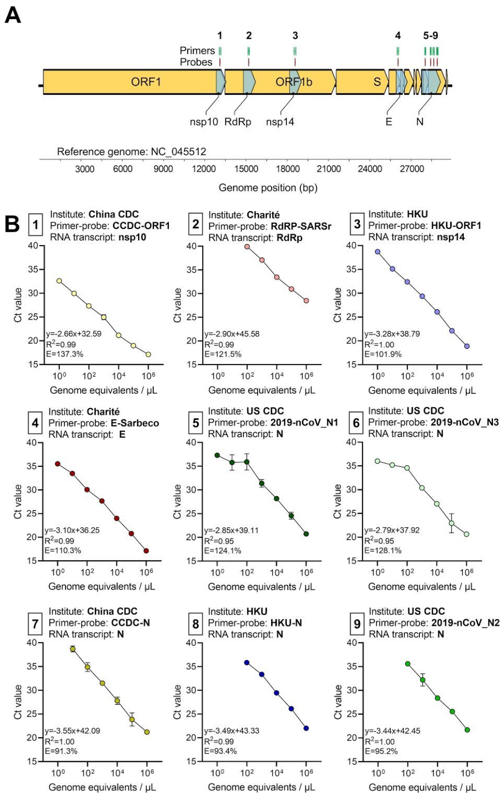
Fig. 1: Generation of RNA transcript standards for validation of SARS-CoV-2 qRT-PCR assays. (A) We reverse-transcribed RNA transcript standards for the non-structural protein 10 (nsp10), RNA-dependent RNA polymerase (RdRp), non-structural protein 14 (nsp14), envelope (E), and nucleocapsid (N) genes to be used for validation of nine primer-probe sets used in SARS-CoV-2 qRT-PCR assays. (B) We generated standard curves for nine primer-probe sets with 10-fold dilutions
