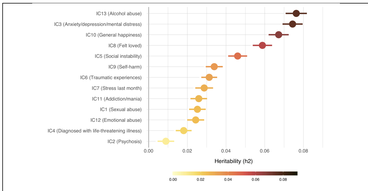
Fig. 2. Heritability estimates of the independent components SNP-based heritability for each IC sorted by decreasing heritability ( h^2 ). Heritability calculated using the LDSC toolbox 36 . Error bars reflect standard errors.
