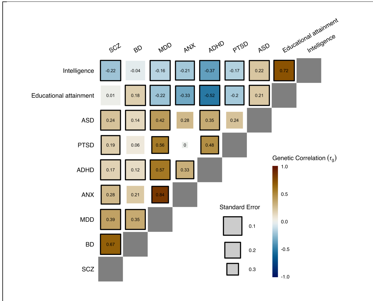
Suppl. Fig. 1. Genetic correlation between the disorders and cognitive traits Numbers inside the boxes denote correlation ( r_g ). Size of the boxes reflect standard error. Significant correlations ( p < FDR ) are indicated with a black border. In line with previous reports 9,25 , the weakest correlation was between PTSD and ANX ( r_g = -0.004 , SE = 0.3408 ) and the strongest between ANX and MDD ( r_g = 0.8441 , SE = 0.1724 ).
