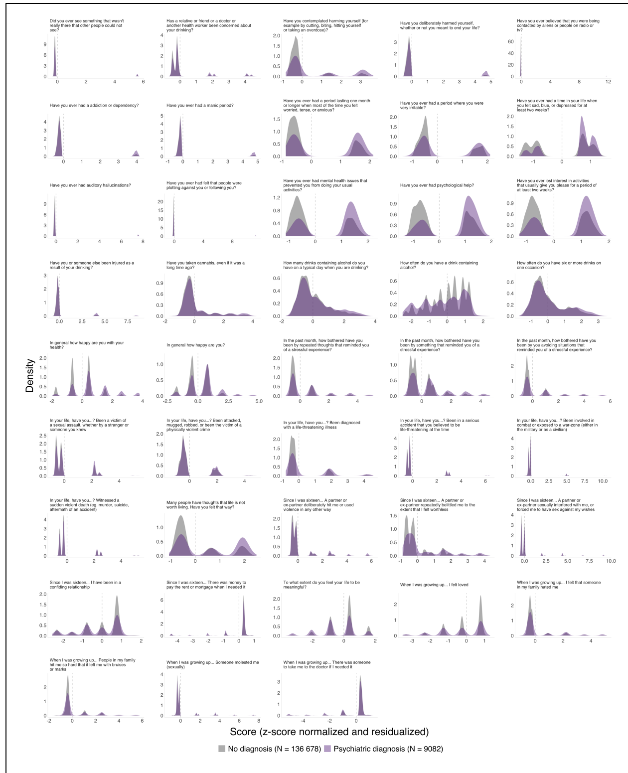
Suppl. Fig. 2. Z-normalized question scores Density plot of the scores comparing the sample of individuals without psychiatric or neurological diagnosis to the individuals with a diagnosed psychiatric disorder. With a few notable exceptions, distributions are fairly similar, supporting that mental health data from healthy individuals can be used to study psychiatric disorders. As expected, in the exceptions
