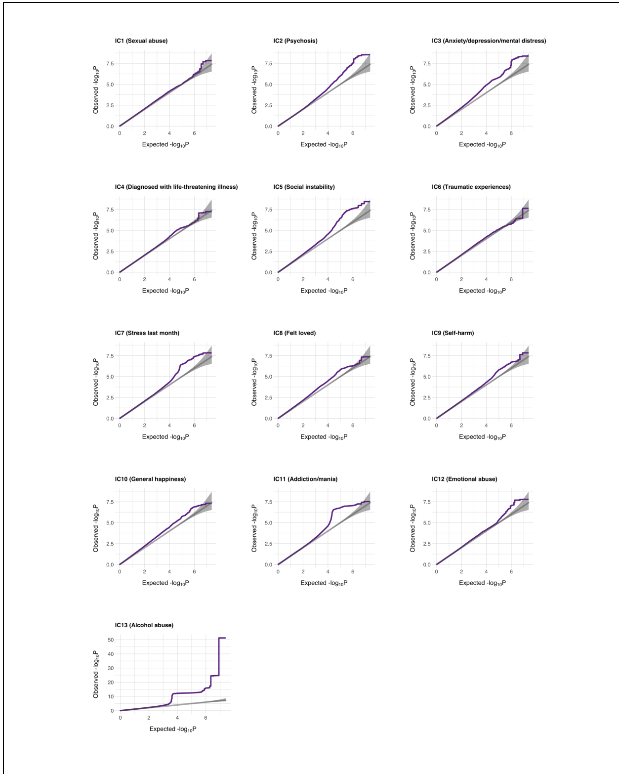
Suppl. Fig. 5. Q-Q plots Q-Q plots showing the genetic signal from each of the ICs. IC13 showed the strongest signal. IC2 showed a strong signal despite having the lowest h^2 . None of the GWAS summary statistics showed any noticeable inflation.
