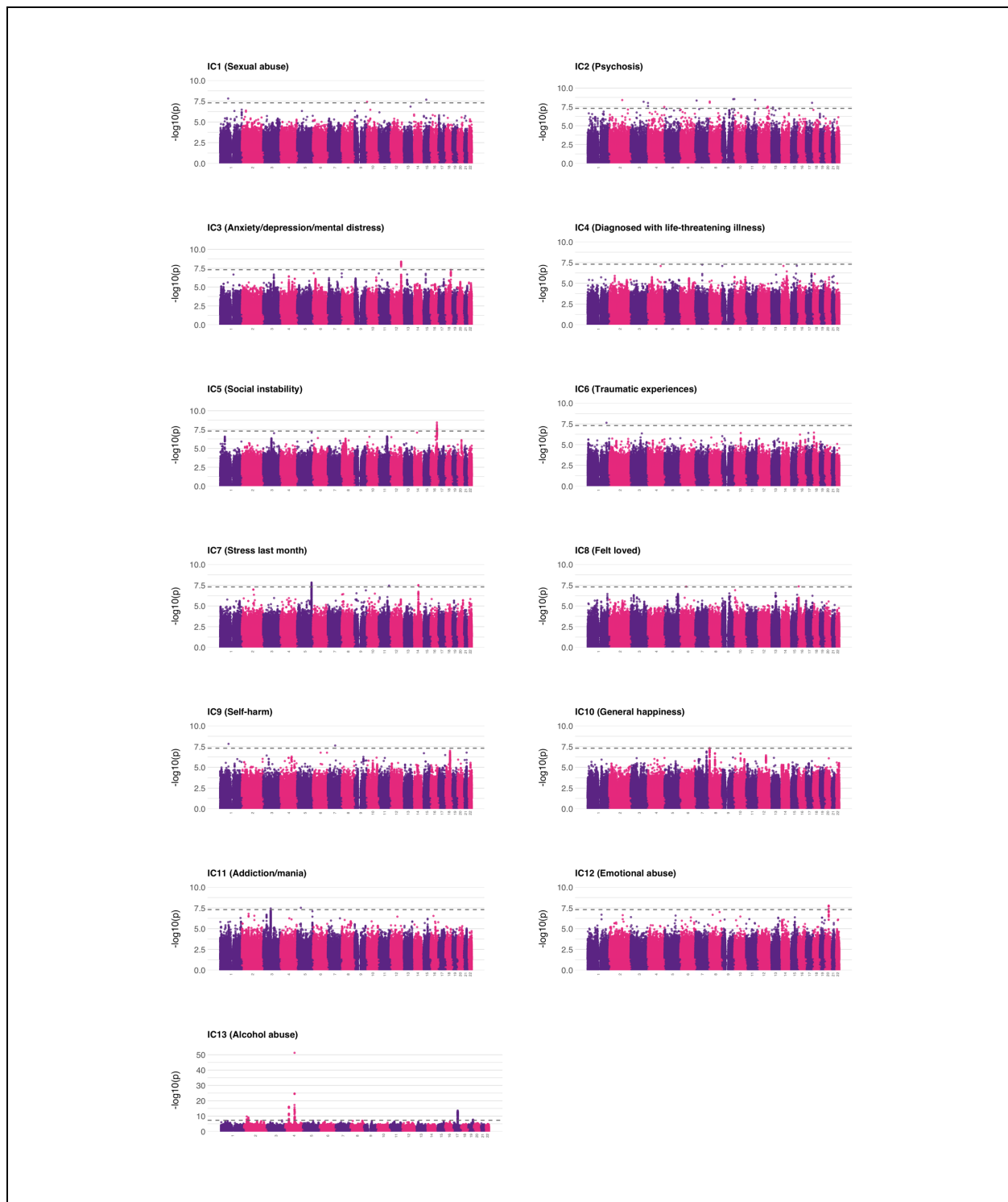
Suppl. Fig. 6. Manhattan plots for the ICs Significance threshold set at 5e-8 . Only IC4 had no genome-wide significant hits, a few more had no lead SNPs, according to FUMA.
