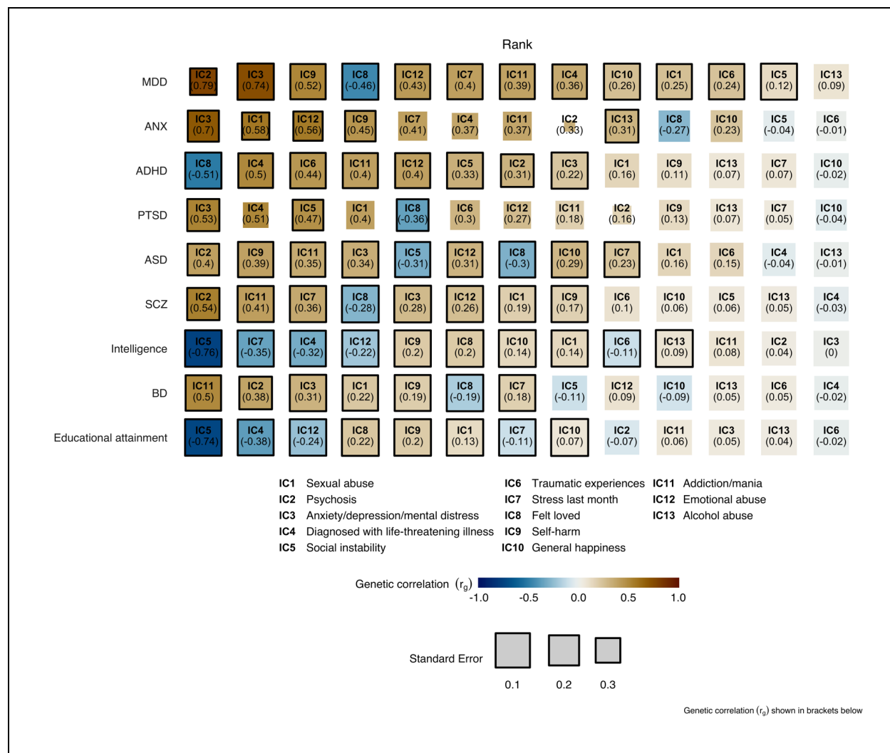
Fig. 3. Genetic correlation between the independent components and disorders and cognitive traits
