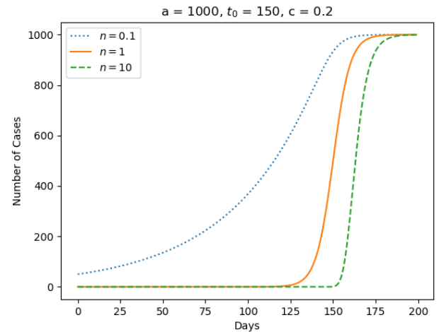
FIG. 4: The plots demonstrate the effect of n on the population growth. n > 1 suggests a growth rate higher than typical logistic function ( n = 1 ) whereas n < 1 suggests a slower growth.
