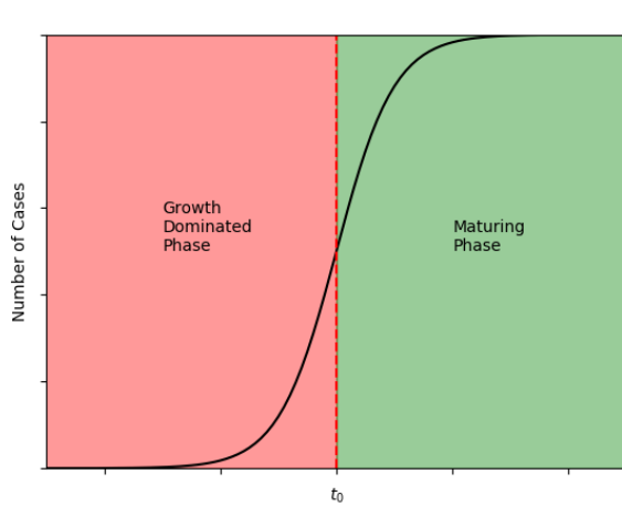
FIG. 1: The classification of countries based on the inflection point. t_0 is the midpoint of the logistic function ( \alpha_E(t_0) = a/2 ) and the turning point where the growth rate begins to slow down.
