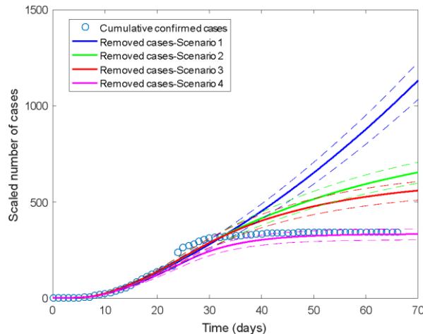
(e) Scaled number of removed cases compared to the cumulative confirmed cases up to March 24 th
