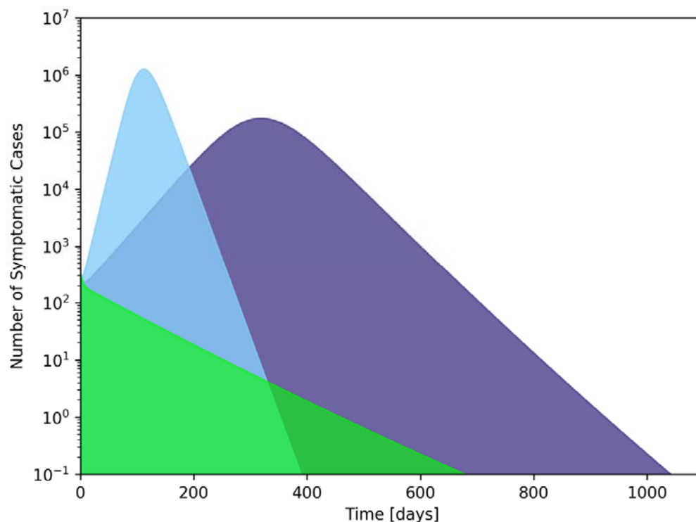
166 167 FIG. 2. Total number of symptomatic cases in Israel from SEQIIR model 168 simulations for 3 scenarios: green – high-efficiency quarantining, purple – medium- 169 efficiency quarantining, light-blue – low-efficiency quarantining.
