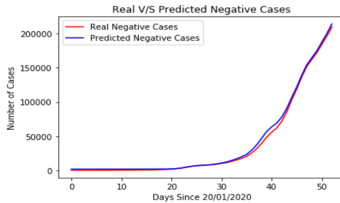
Figure 8. Real case V/s Predicted Negative Case using LSTM-GRU RNN
