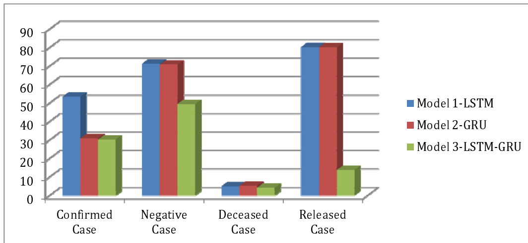
Figure 6. RMSE Comparison among these three models with along with the cases.
