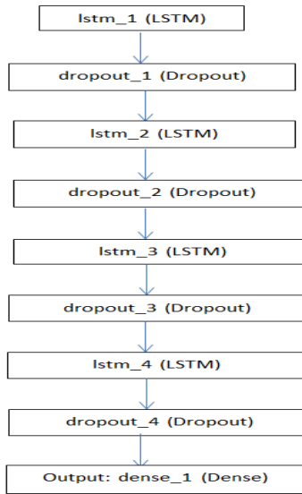
Figure 2. Neural network structure for model 1
