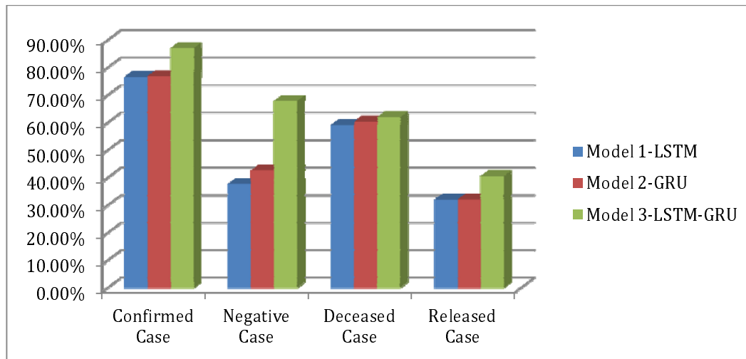
Figure 5. Accuracy Comparison among these three models with along with the cases.
