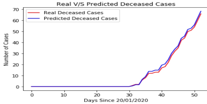
Figure 9. Real V/s Predicted Deceased Case using LSTM-GRU RNN
