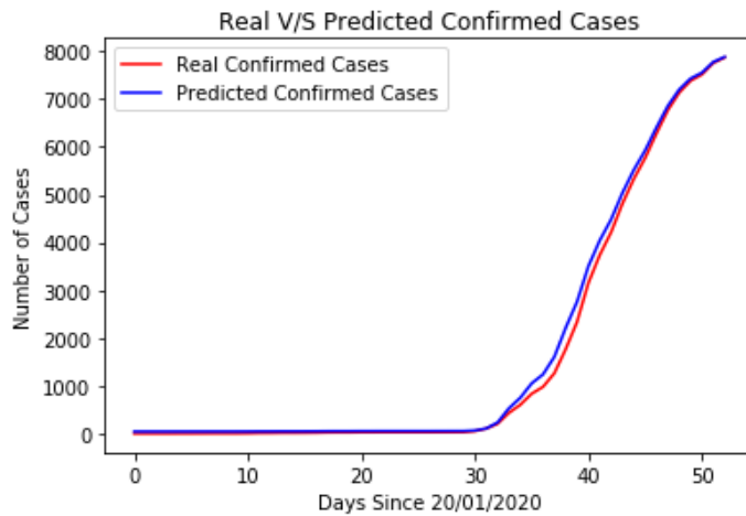
Figure 7. Real V/s Predicted Confirmed Case using LSTM-GRU RNN
