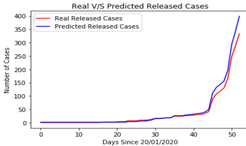
Figure 10. Real V/s Predicted Released Case using LSTM-GRU RNN
