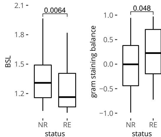
Figure 2: Predicted phenotypic differences between responder and non-responder microbiomes. Combined data sets ERP013257, SRP135559, ERP116682 and SRP102742, 46 patients, 159 samples. BSL: predicted average biological safety level of the microbiome. NR: non-responders, RE: responders. Numbers reflect Wilcoxon signed rank test continuity corrected p-values.
