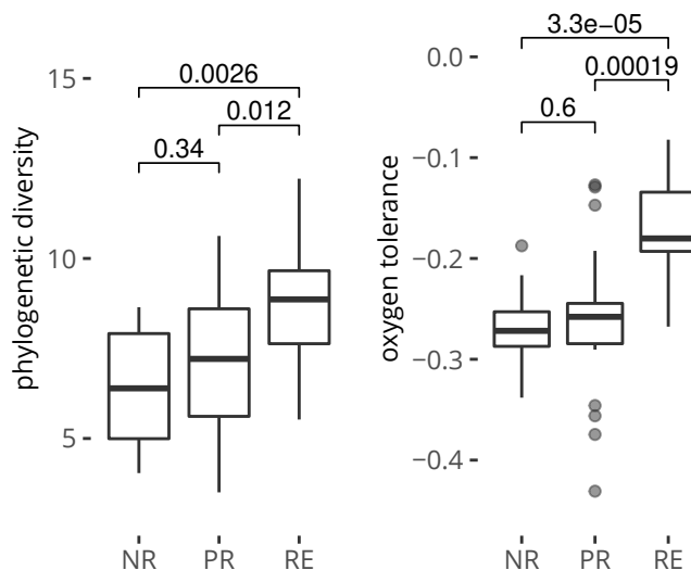
Figure 4: Donor microbiome phenotypes, data set ERP013257. 51 samples from 12 donors. Numbers reflect Wilcoxon signed rank test continuity corrected p-values. Donors are associated with NR: non-responders, PR: partial responders, RE: responders.
