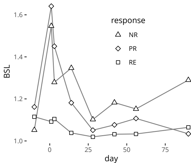
Figure 3: BSL trajectory across antibiotics course, FMT and follow-up. Data set ERP013257, 13 patients. Data points reflect the median predicted biological safety levels per response group. NR: non-responders, PR: partial responders, RE: responders. Antibiotics course: days -10 to 0, FMT: day 1.
