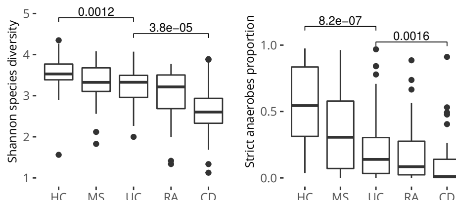
Figure 1: Microbiome phenotypes in IMIDs. Data set SRP183770, 79 subjects, 201 samples. Numbers reflect Wilcoxon signed rank test continuity corrected p-values. HC: healthy controls, MS: multiple sclerosis, UC: ulcerative colitis, RA: rheumatoid arthritis, CD: Crohn's disease.
