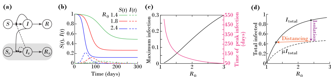
Figure 1: Model and predictions. (a) Extended susceptible-infected-removed/recovered (SIR) model. S , I , and R are proportions of susceptible, infected, and recovered individuals, respectively. Subscript v represents vulnerable individuals. (b) Solutions of the SIR model with R_0 = 1.4, 1.8, and 2.4 . Solutions S and I represent the fractions of the susceptible and infected populations over time. Initial conditions: S = 0.9999, I = 0.0001, and R = 0 . (c) Maximum fraction of infected individuals (left axis) and time at which the fraction of infected individuals has its peak (right axis). (d) Continuous curve: total infected fraction I_{\text{total}} = 1 - S(\infty) versus R_0 . Dashed curve shows an example of reducing the exponent in (3) by decreasing \mu by a factor 2 through targeted isolation. Arrows show that the infected vulnerable population can be reduced by distancing and isolation.
