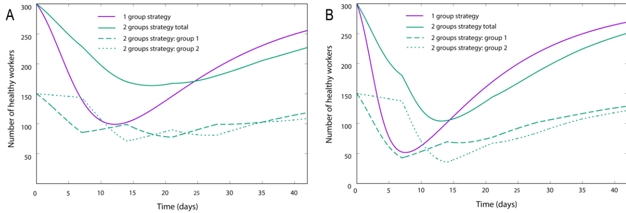
Figure 5. Representative examples of infection rates of healthcare workers with and without desynchronization (SLIRW). Number of healthy workers (susceptible plus recovered) as a function of time.
