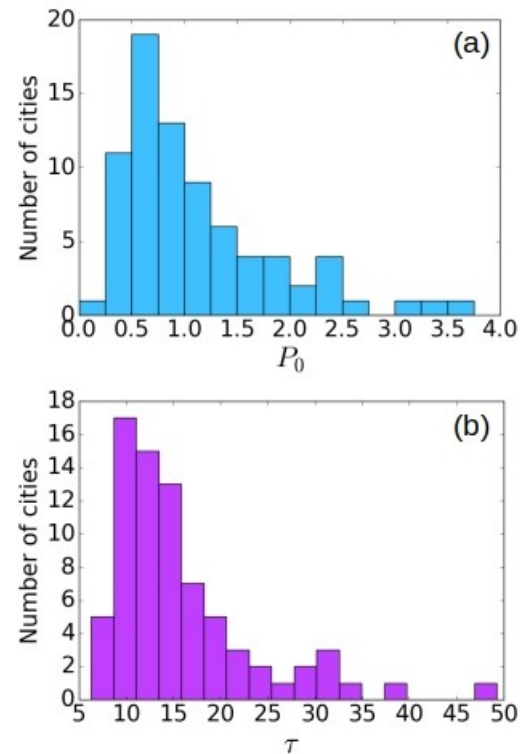
FIG. 4: Statistical properties of the two-stages city infection with latency period of 4 days. (a) The constant infection rate, P_0 is mostly range 0.5-2 while in a few cities it can be much larger. The average value is 1.16 with standard deviation 0.84. (b) The distribution of the exponent \tau characterizing the extinction of the disease which found to be in the range 5-50 days. The average value is 15.9 with standard deviation 7.7.
