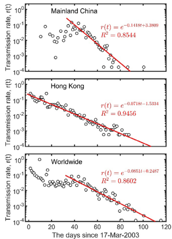
Fig.3: The exponential damping of the 2003 SARS transmission rate in China. Data from the website of WHO ( www.who.int ).
