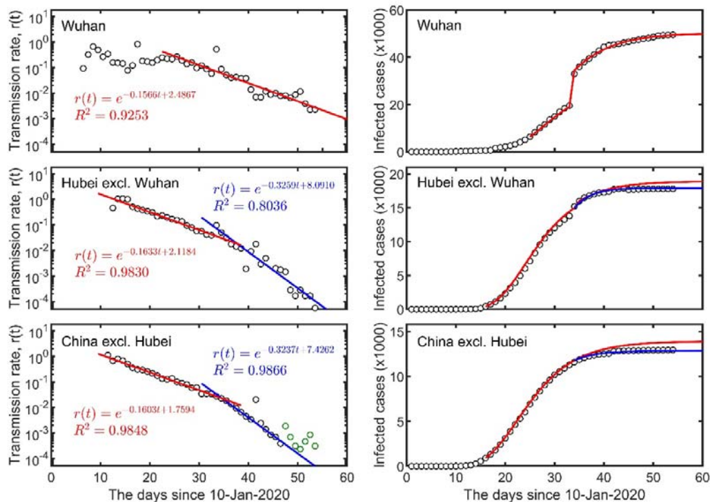
Fig.1: The exponential damping of COVID-19 transmission rates in Wuhan city, Hubei Province (excluding Wuhan) and the rest of China (excluding Hubei) (left column), and the total number of infection cases (right column). The red lines on the left panel represent regressions of the data after 3-Feb-2020 for Wuhan city, from 25-Jan-2020 to 11-Feb-2020 for Hubei province (excluding Wuhan) and the rest of China (excluding Hubei), while blue lines are from regressions based on the data after 12-Feb-2020. The lines on the right panels are the corresponding predictions using the fitted time-dependent transmission rate ( r(t) ). Circles indicate real data, where green circles indicate cases imported from other countries and were not considered in the regression.
