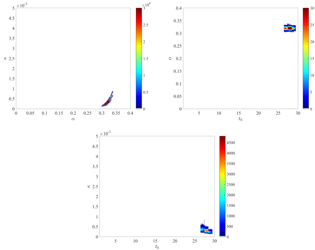
Figure A1: Joint posterior distributions of (\alpha, \kappa) , (t_0, \alpha) and (t_0, \kappa) .
