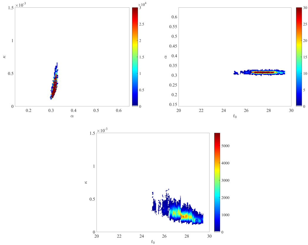
Figure A2: Joint posterior distributions of (\alpha, \kappa) , (t_0, \alpha) and (t_0, \kappa) obtained with a more informative prior.
