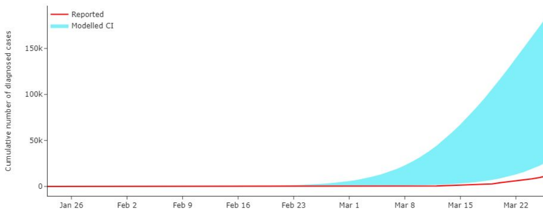
Figure 15: An overlay of modelled confidence interval for the number of diagnosed cases and reported values in the UK. The model overestimates the number diagnosed cases since March 15th. This may be caused by flight-related interventions introduced since January, which in case of the geographically isolated country like the UK may have stronger impact than similar restrictions in countries from the continental part of Europe.
