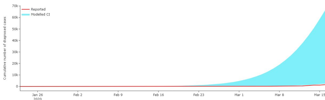
Figure 18: An overlay of modelled confidence interval for the number of diagnosed cases and reported
