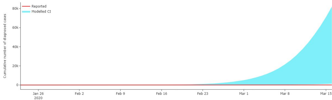
Figure 19: An overlay of modelled confidence interval for the number of diagnosed cases and reported values in Vietnam. The limited number of tests carried in the country (only 24 per 1 mln citizens) leads to locally reduced tDR (proportion of detected to undetected cases), which possibly became smaller than the tDR value assumed in the model (0.0061) and caused the observed overestimations of the model.
