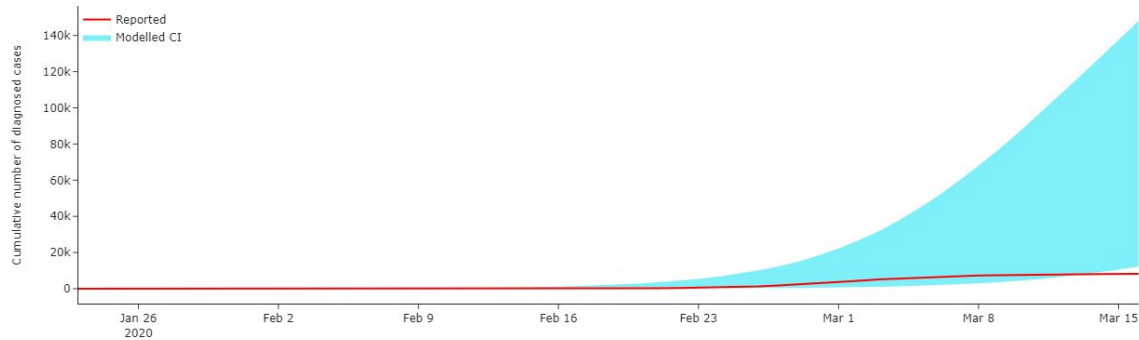
Figure 14: An overlay of modelled confidence interval for the number of diagnosed cases and reported values in the Republic of Korea. The model overestimates the number of diagnosed cases at the end of the tested period, even though the Republic of Korea excels in the number of carried tests (4099 per million people) and should have locally increased tDR (proportion of diagnosed to undiagnosed cases). Most likely, this discrepancy is caused by the fact that the model does not take into account precautions overtaken by the Korean government that seem to successfully slow down the spread of the disease.
