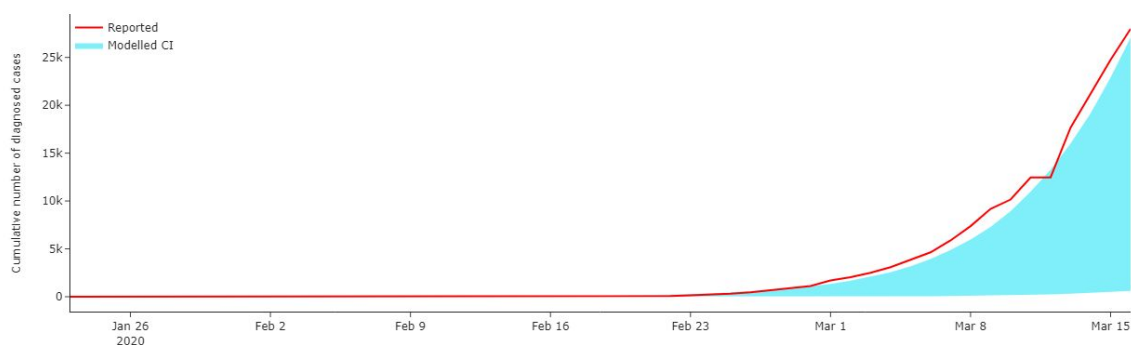
Figure 12: An overlay of modelled confidence interval for the number of diagnosed cases and reported values in Italy. The model underestimates this number which may be explained either by a relatively large number of tests carried recently in Italy (1005 per million of people) leading to larger tDR (proportion of diagnosed to undiagnosed cases) than used in our model, or by a higher than typical pace of epidemic development.
