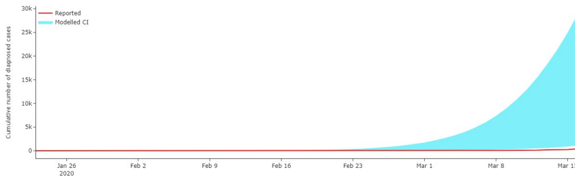
Figure 8: An overlay of modelled confidence interval for the number of diagnosed cases and reported values in Canada. The number of tests carried in Canada was not reported in our sources, but the fact that the model overestimates the number of diagnosed cases, we suspect that it is relatively small, leading to locally reduced tDR (proportion of diagnosed to undiagnosed cases) in relation to the value used in our simulation (0.0061). Another possible explanation is that precautions introduced by the Canadian government successfully slowed down the epidemic.
