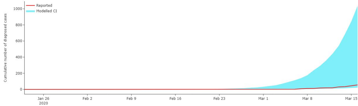
Figure 4: An overlay of modelled confidence interval for the number of diagnosed cases and reported values in Argentina. The predictions of the model agree with observations.
