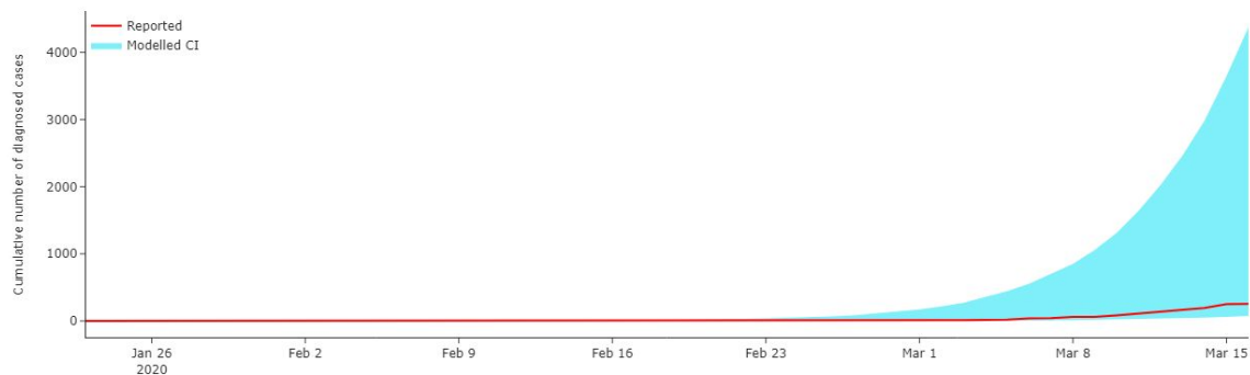
Figure 11: An overlay of modelled confidence interval for the number of diagnosed cases and reported values in Israel. The predictions of the model agree with observations.
