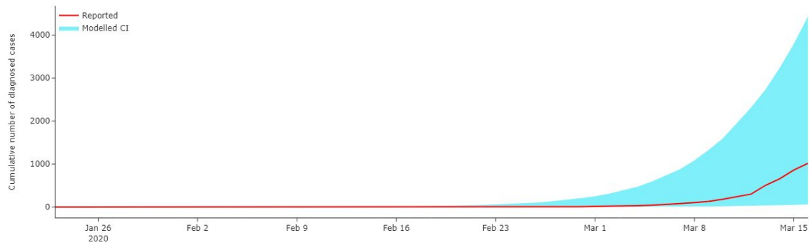
Figure 5: An overlay of modelled confidence interval for the number of diagnosed cases and reported values in Austria. The predictions of the model agree with observations.
