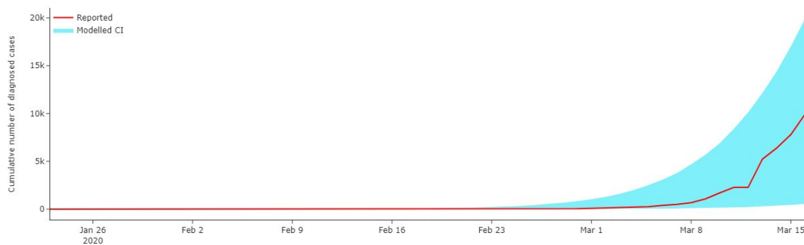
Figure 17: An overlay of modelled confidence interval for the number of diagnosed cases and reported values in Spain. The predictions of the model agree with observations.
