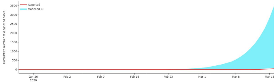
Figure 16: An overlay of modelled confidence interval for the number of diagnosed cases and reported values in Mexico. The number of tests carried in Mexico was not reported in our sources, but the fact that the model slightly overestimates the number of diagnosed cases, we suspect that it is relatively small, leading to locally reduced tDR (proportion of diagnosed to undiagnosed cases) in relation to the value used in our simulation (0.0061).
