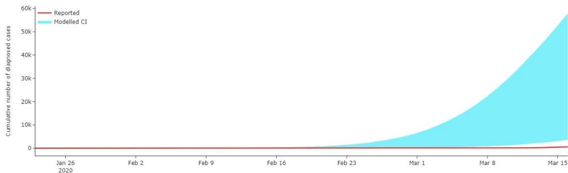
Figure 15: An overlay of modelled confidence interval for the number of diagnosed cases and reported values in Malaysia. The limited number of tests carried in the country (only 97 per 1 mln citizens) leads to locally reduced tDR (proportion of detected to undetected cases), which possibly became smaller than the tDR value assumed in the model (0.0061) and caused the observed overestimations of the model.
