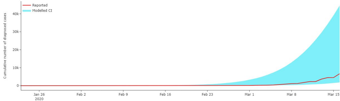
Figure 9: An overlay of modelled confidence interval for the number of diagnosed cases and reported values in France. The predictions of the model agree with observations.
