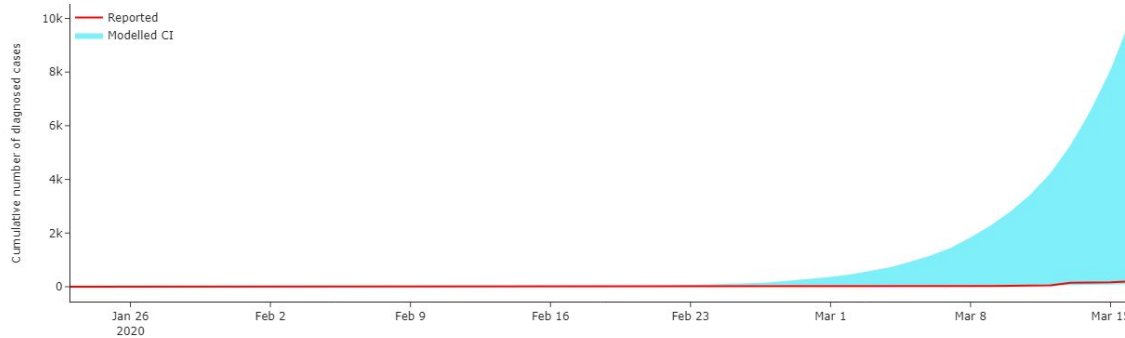
Figure 7: An overlay of modelled confidence interval for the number of diagnosed cases and reported values in Brazil. The predictions of the model agree with observations.
