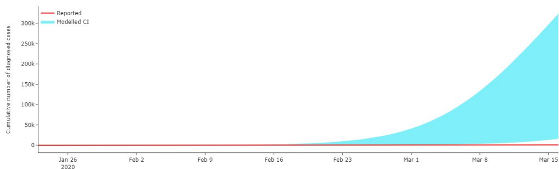
Figure 13: An overlay of modelled confidence interval for the number of diagnosed cases and reported values in Japan. The limited number of tests carried in the country (only 76 per 1 mln citizens) leads to locally reduced tDR (proportion of detected to undetected cases), which possibly is smaller than the tDR value assumed in the model (0.0061) and caused the observed overestimations of the model.
