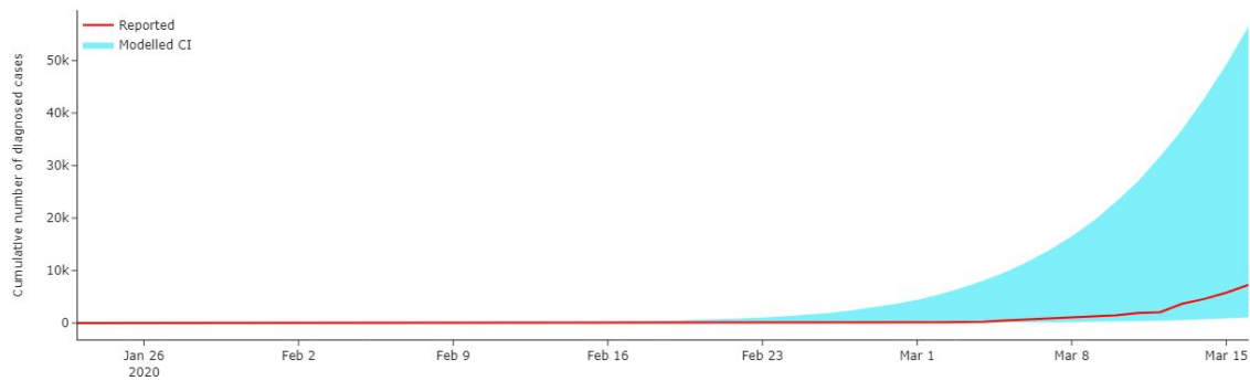
Figure 10: An overlay of modelled confidence interval for the number of diagnosed cases and reported values in Germany. The predictions of the model agree with observations.
