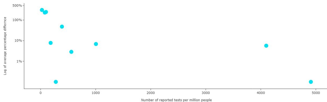
Figure 3: Average percentage difference (logged) between modelled and observed number of detected cases juxtaposed with number of reported tests per million people in selected countries of known number of tests (see Table 2 for details). These values are negatively correlated with Spearman correlation coefficient of 95% CI ranging from -0.291 to -0.945 and (n=10).
