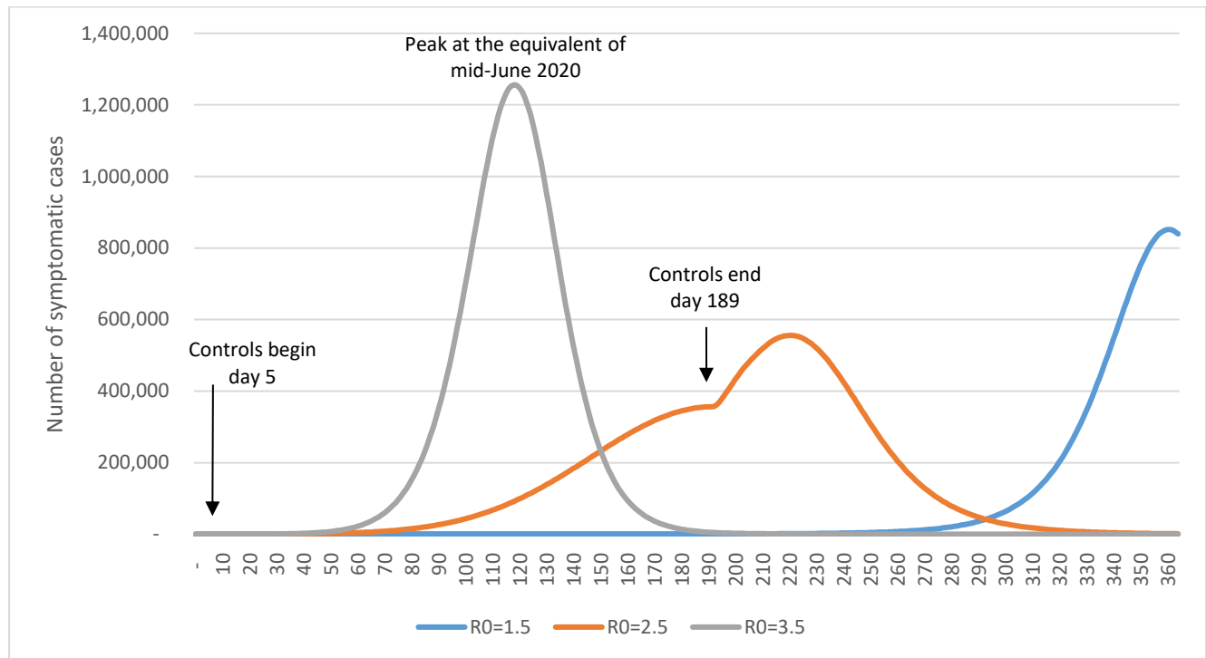
Figure 1: Numbers of prevalent symptomatic COVID-19 cases by day for the R_0 = 1.5, 2.5, and 3.5 scenarios and all with 25% of “general contact reduction” as modelled using CovidSIM (unrecognised introduction of the infection occurs at time 0; control measures begin at day 5 and end six months later i.e., on day 189).
