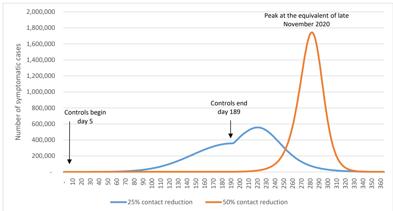
Figure 2: Numbers of prevalent symptomatic COVID-19 cases by day for the R_0 = 2.5 scenarios and different levels of general contact reduction as modelled using CovidSIM (unrecognised introduction of the infection occurs at time 0; control measures begin at day 5 and end six months later i.e., on day 189).
