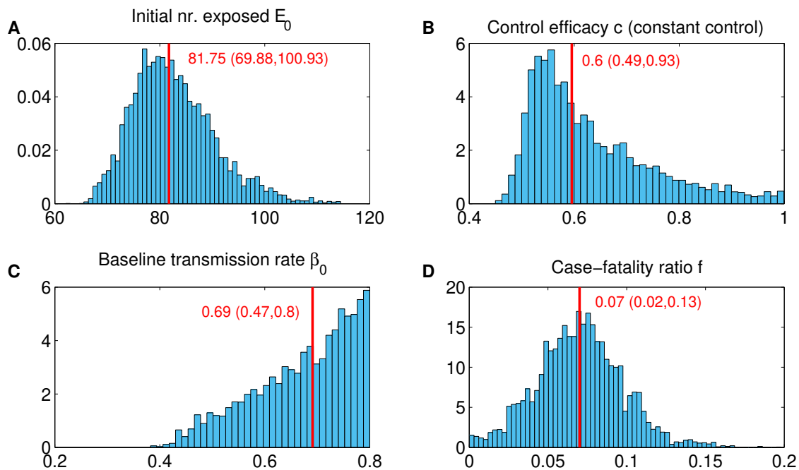
Figure S2: Parameter posterior distributions for model assuming constant control ( T_{in} = 5 ) based on fitting data March 9-28.
