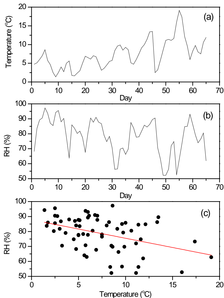
Figure 1. (a) Mean daily meteorological temperature, and (b) relative humidity (RH) in Wuhan, China for the period from 1 January to 6 March, 2020. (c) Plot of the relative humidity versus temperature, showing negative correlations ( \rho = -0.42 ).
