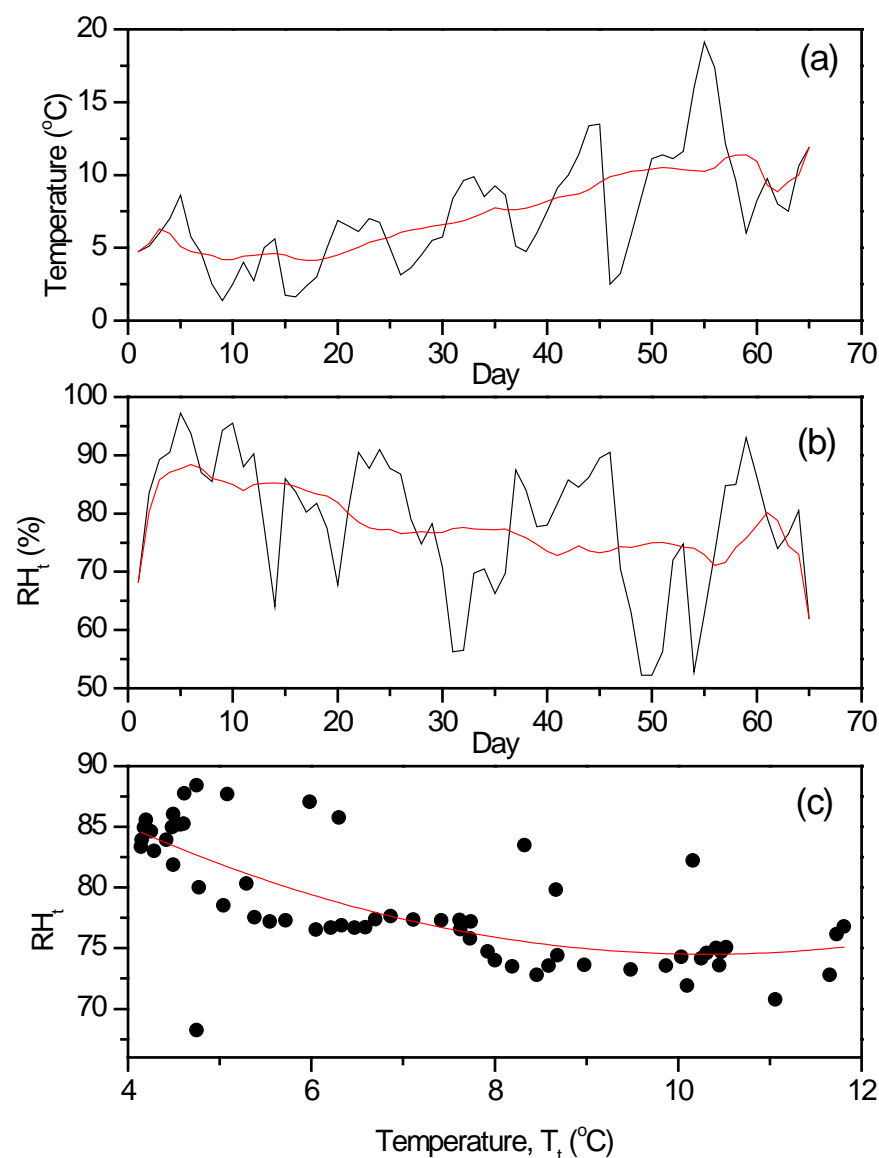
Figure 4. Meteorological (a) temperature, and (b) relative humidity in Wuhan, China, for the period from 1 January to March 6, 2020. The red lined depict the long-term trend obtained by 15-days moving average filtering. (c) Plot of the trend relative humidity and the trend temperature. A negative correlation between these trends can be observed.
