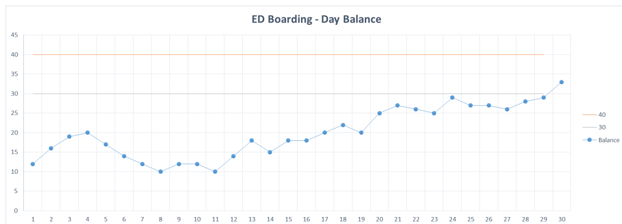
Figure 2: Simulation which doesn't cross threshold
