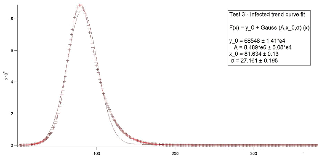
Figure 2: Test 3 – Italy infected trend, gaussian curve fit.
