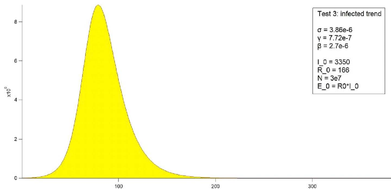
Figure 1: Test-3 – Italy infected trend.
