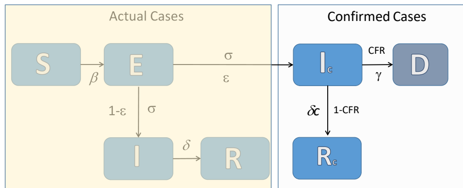
Figure 1: A schematic of the proposed compartmental SEIRD model. The actual number of cases is unknown.
