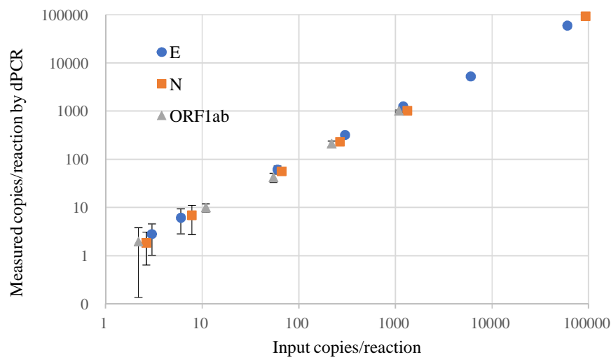
Figure 1. Validated range of the dPCR assays for E, ORF1ab and N gene. Evaluation of linearity of samples containing E, ORF1ab and N gene molecules over the extended \lambda range ( 0.0002 < \lambda < 7.83 ). Data are shown in mean with standard deviation for each dilution series ( 3 \leq n \leq 10 ).
