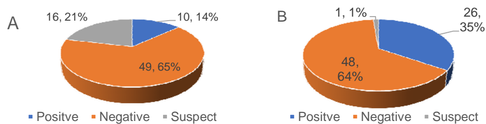
Figure 3. Diagnostics of SARS-CoV-2 by RT-qPCR and dPCR on 75 close contacts. 10 positive, 49 negative and 16 suspected were reported by RT-Qpcr (A). 26 positive, 48 negative and 1 equivocal were determined by dPCR (B).
