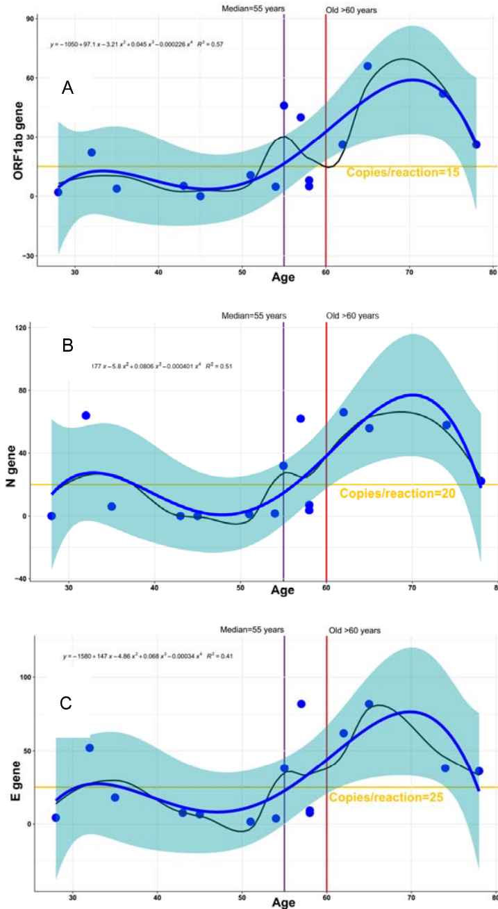
Figure 4. Correlation analysis between age and target gene copy number of ORF1ab (A), N (B) and E (C). The horizontal line representing the threshold of 15, 20 and 25 copies/reaction for ORF1ab, N and E, respectively. The ORF1ab, N and E gene copy number were higher than their threshold for 100% patients elder than 60 and 75% (6 out of 8 patients) elder than 55 (the median).
