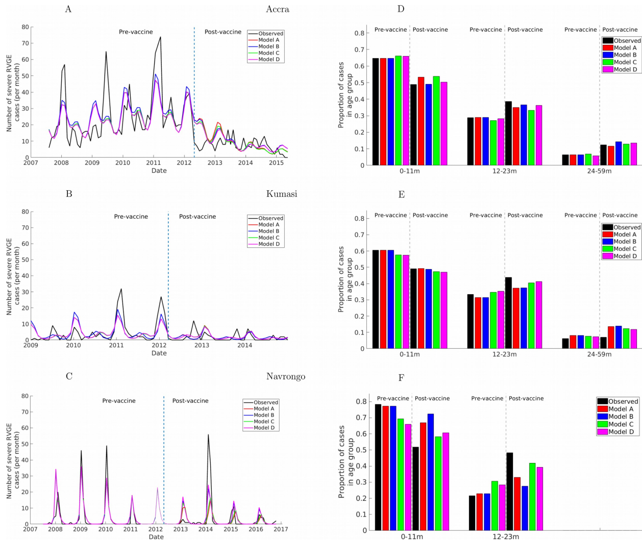
Fig. 3. Fit of models to the observed data. (Left) Model-predicted and observed monthly incidence of severe RVGE cases among children during both pre- and post-vaccine periods. The vertical line indicates the date of vaccine introduction (April 2012). (Right) Model-predicted and observed proportion of severe RVGE in each age group before and after vaccine introduction. The grey dashed lines separate the pre- and post-vaccination distribution for each age group. The light line region of C indicates model predictions for Navrongo for the period with missing data.
