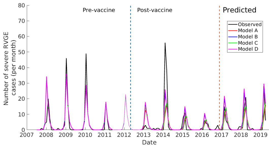
Fig. 4. Comparison of model and observed rotavirus incidence in Navrongo showing both models fitting and evaluation periods. The brown vertical line separates the model fitting period from the evaluation period.
