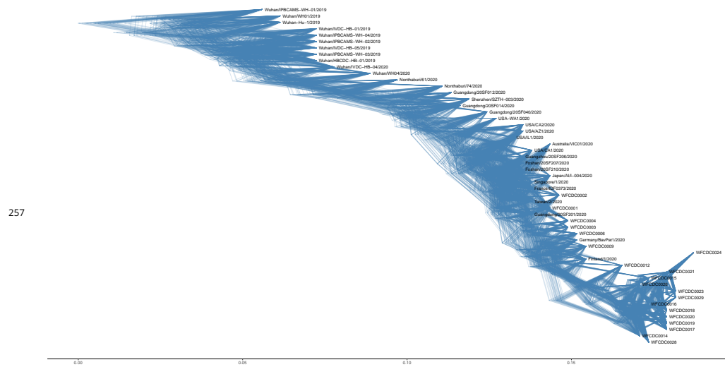
Figure 1-Figure supplement 2. A tree density plot based on the posterior distribution of trees computed in BEAST2.
