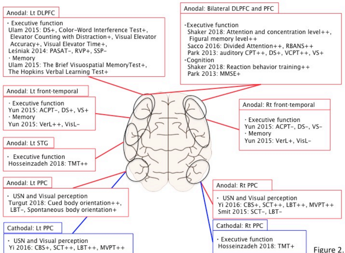
Figure 2. Relationship between stimulation site and neuropsychological test results in tDCS:
