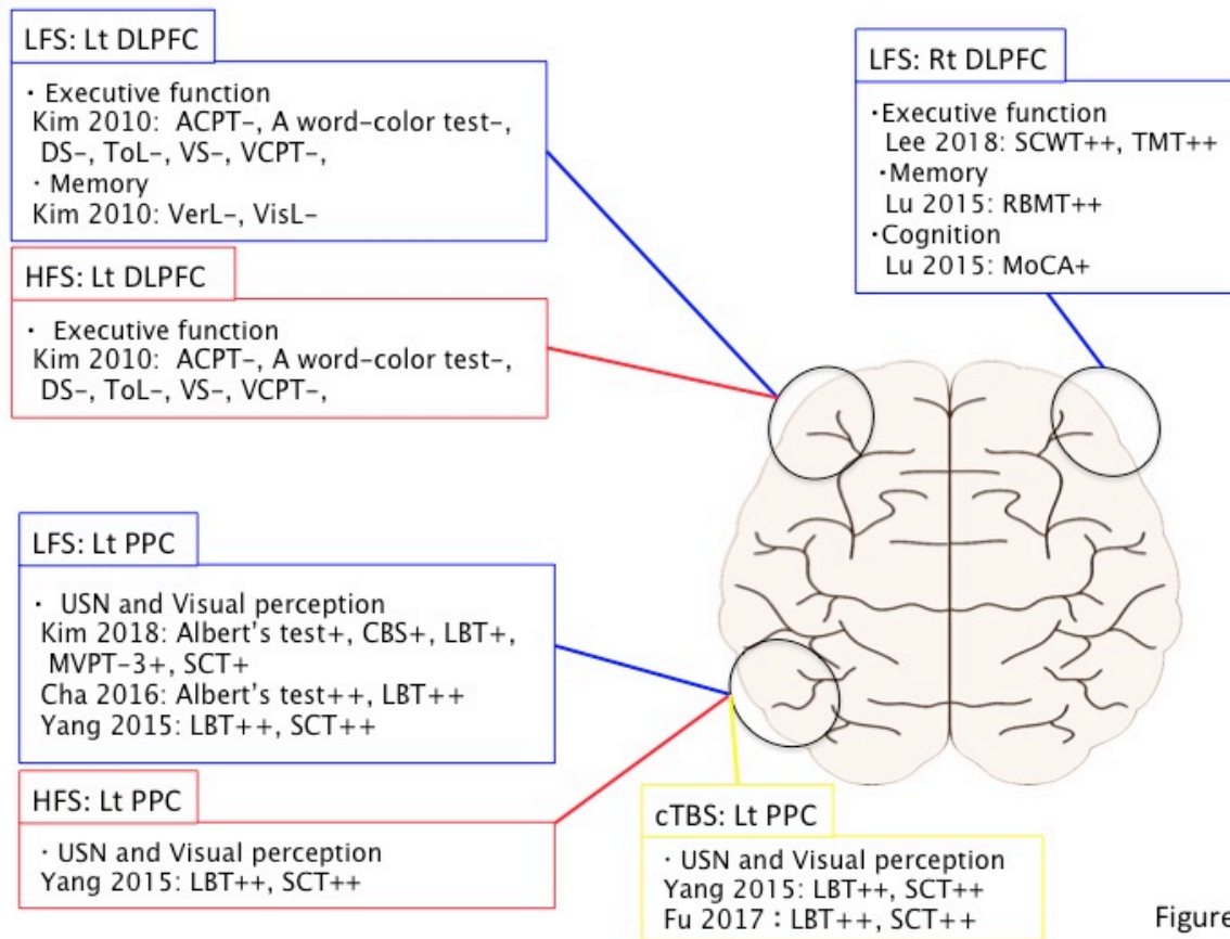
Figure 1. Relationship between stimulation site and neuropsychological test results in rTMS:
