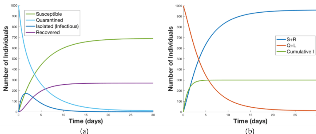
FIGURE 5. In the numeric solution for our SEIR Model with a quarantine-all policy enacted, the population of each compartment versus time, which notably does not include an exposed compartment, is shown in (a). In (a) are individuals suspected to be exposed and quarantined initially, until they either fall ill (and are isolated) or are released after the quarantine duration (21 days). The active working ( S + R ) and inactive ( Q + L ) populations versus time with the cumulative infections versus time are shown in (b). The quarantine-all policy has very effectively reduced the total number of disease cases but has vastly increased the burdens of quarantine and isolation.
