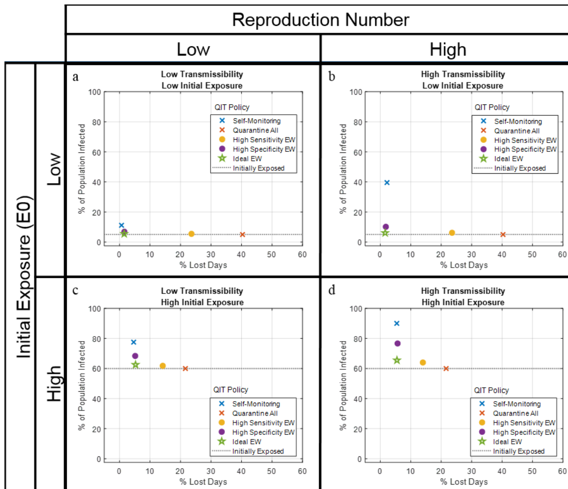
FIGURE 11. The trade space for the percentage of population infected versus percentage of lost duty days compares the augmented policies: self-monitoring, quarantine-all, and quarantine-on-alert with three levels of early warning performance (high sensitivity, high specificity, and ideal early warning). Four situations were considered: low-transmissibility pathogen with a low initial exposure (a), high-transmissibility pathogen with a low initial exposure (b), low-transmissibility pathogen with a high initial exposure (c), and high-transmissibility pathogen with a high initial exposure (d).
