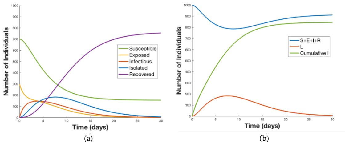
FIGURE 4. In this numeric solution for our SEIR model with a self-monitoring and isolation policy enacted, the population of each compartment versus time is shown in (a), and the active working ( S + E + I + R ) and inactive ( L ) populations versus time with the cumulative infections versus time are shown in (b). The self-monitoring policy has effectively reduced the total number of disease cases and blunted the outbreak's peak severity (number of cases in I and L peak at approximately 7 days).
