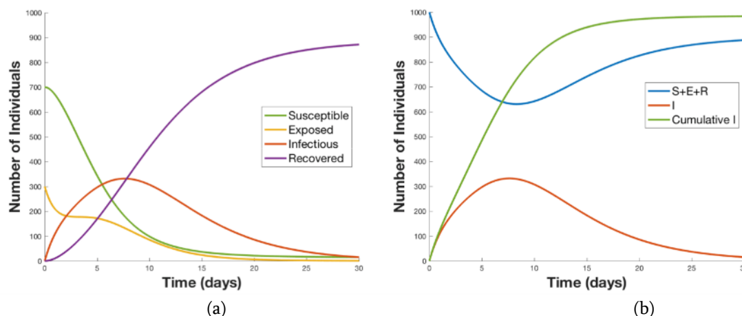
FIGURE 2. A numeric solution for the baseline SEIR model shows the population of each compartment versus time (a), which indicates that for an initial exposure of 300 individuals, nearly the entire population will eventually fall ill; the cumulative number of infections (Cumulative I) versus time is shown in (b).
