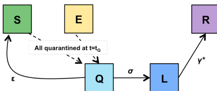
FIGURE 5. The model diagram for a quarantine-all policy moves all susceptible and exposed individuals to the quarantined compartment ( Q ) at the time t_Q . Quarantined individuals who do not develop symptoms are returned to the susceptible compartment after a maximum incubation time.
