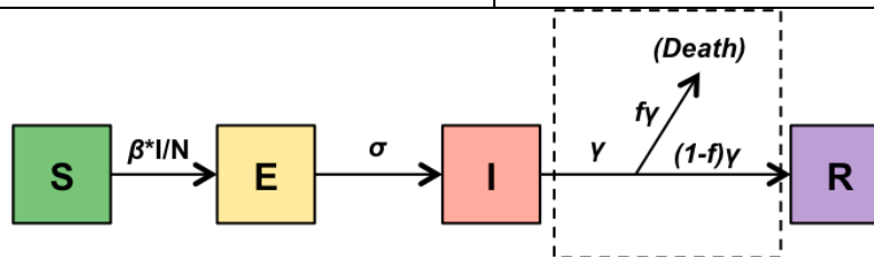
FIGURE 1. In this schematic diagram of the SEIR model, each box represents a compartment of the population, and arrows show the progression of individuals through those compartments. Expressions above arrows are rate coefficients showing progression through compartments. Note that the dashed boxed portion, indicating individuals leaving the population because of death, will not be included in future diagrams for simplicity.
