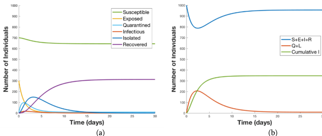
FIGURE 7. This numeric solution for our SEIR model with a quarantine-on-alert policy enacted shows the population of each compartment versus time (a); the plot shows how such an early warning technology could limit the outbreak size. As the initially exposed individuals receive alerts, they enter the quarantine-on-alert compartment and are unable to infect the susceptible compartment. The active working ( S + E + I + R ) and inactive ( Q + L ) populations versus time are shown with the
