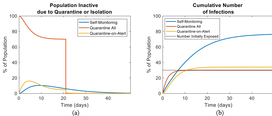
FIGURE 9. The model outputs compare consequences of self-monitoring, quarantine-all, and quarantine-on-alert outbreak response policies. In (a), the plot shows the number of inactive individuals that are unable to work due to quarantine and isolation (Q + L for quarantine-all and quarantine-on-alert, only L for self-monitoring because it does not utilize quarantine) versus time. The sharp drop-off for quarantine-all represents the release of all quarantined individuals after 21 days. In (b), the plot shows the cumulative infections versus time. Any infections above the dotted line (number of individuals initially exposed at t = 0 ) indicate additional transmission of the pathogen.
