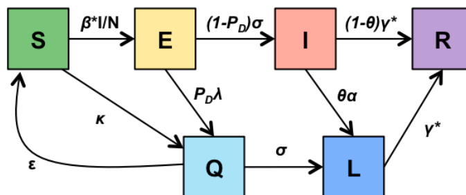
FIGURE 6. This hybrid model diagram illustrates the final quarantine-on-alert policy. The performance of the PRESAGED-like early warning system is now explicitly added, including the probabilities of early detection and false alarm, as well as an expected early detection time before symptom onset and infectiousness. This hybrid between quarantine-all and self-monitoring with isolation seeks to leverage the epidemic-limiting behavior of both policies while reducing the cost and burdens of each.
