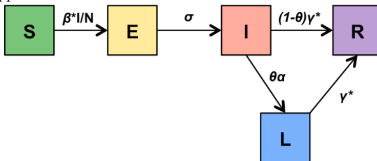
FIGURE 3. The model diagram for a self-monitoring and self-reporting policy includes an additional compartment ( L ) for individuals who are isolated after developing symptoms. Note that fatalities are left out for simplicity.
