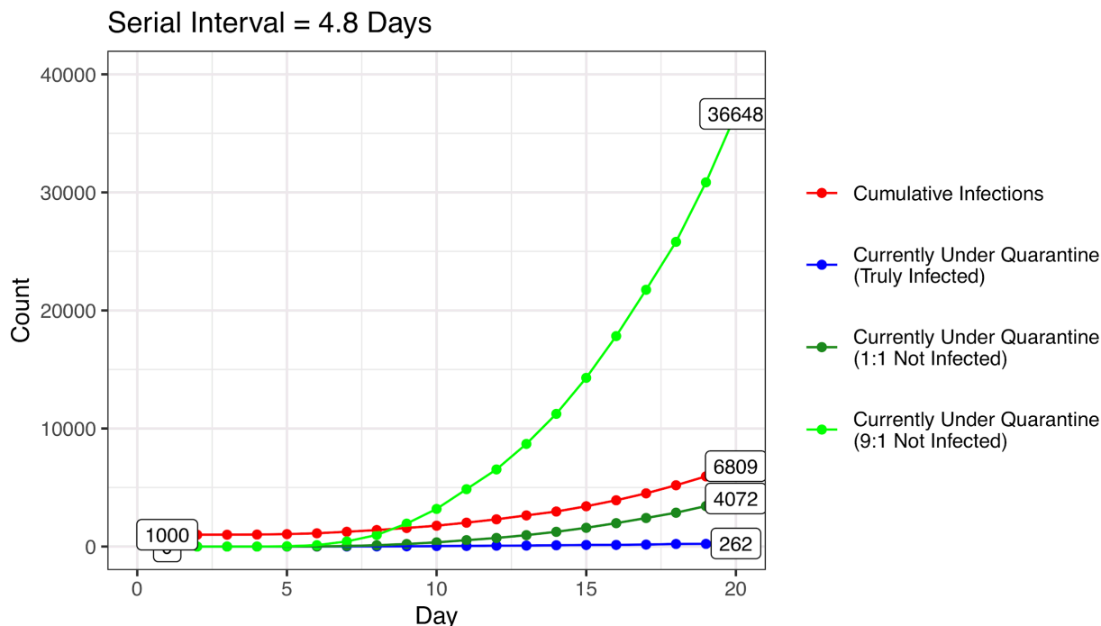
Figure 1: Simulated daily growth of infections and individuals under quarantine
