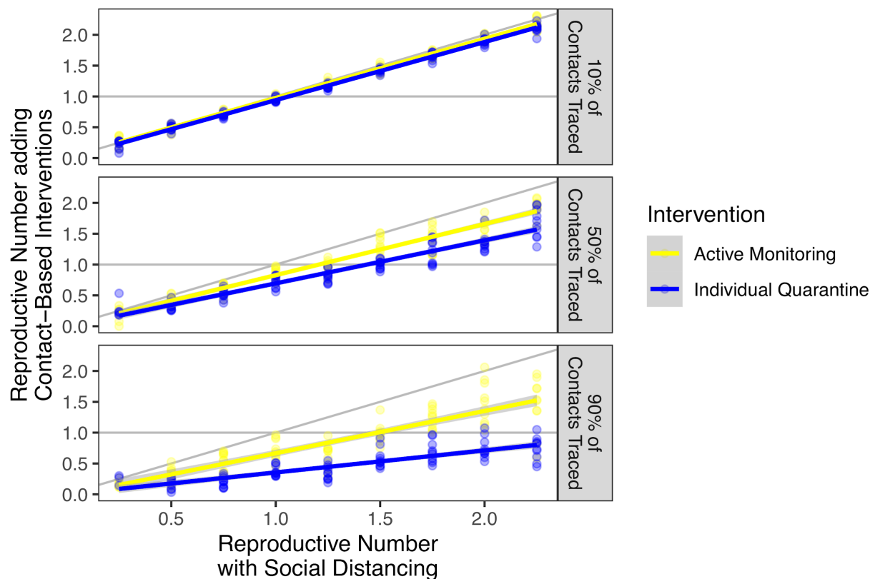
Figure 5: Synergistic effect of social distancing and interventions targeted by contact tracing
