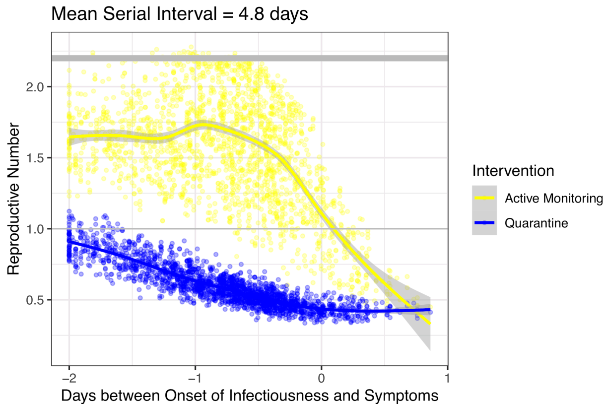
Figure 3: Impact of presymptomatic infectiousness on effective reproductive number
