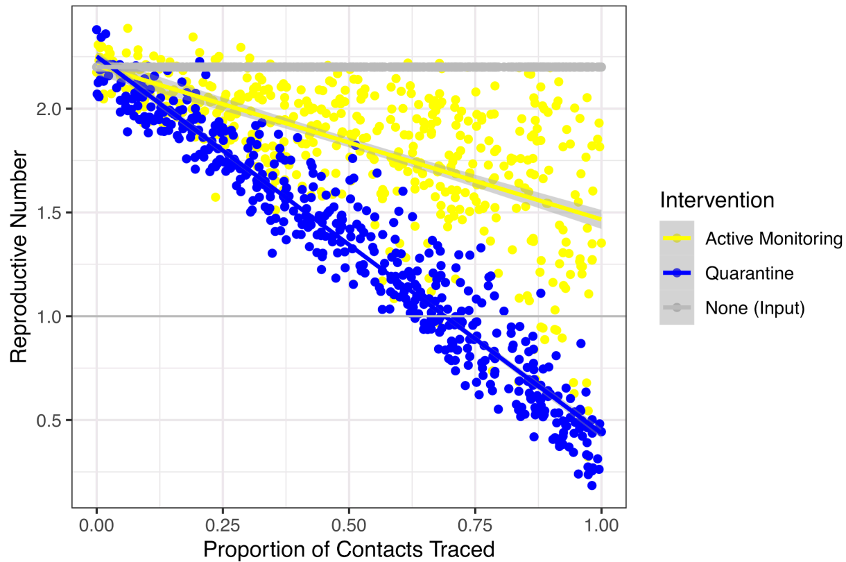
Figure 4: Impact of proportion of contacts traced on effective reproductive number
