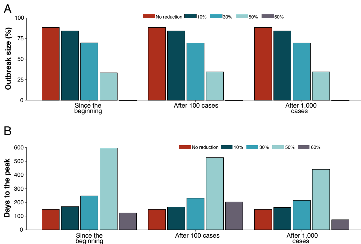
FIG. 8: Effect of a reduction in transmission on the (A) outbreak size and (B) time for the disease to peak. The simulated reductions are as indicated in the legends and have been implemented either from the onset of the outbreak or when a certain number of cases in the whole country are detected. Once the transmissibility is reduced by 60% or more, the epidemic fades out. Note that reducing the transmissibility always delays the spreading, except in situations where the disease dies out, for which the peak occurs earlier.
