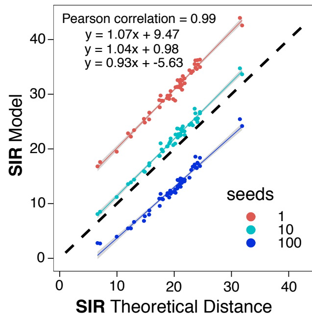
FIG. 10: Relationship between the hitting time in a simulation of SIR dynamics in our metapopulation and the theoretical one for different number of seeds.
