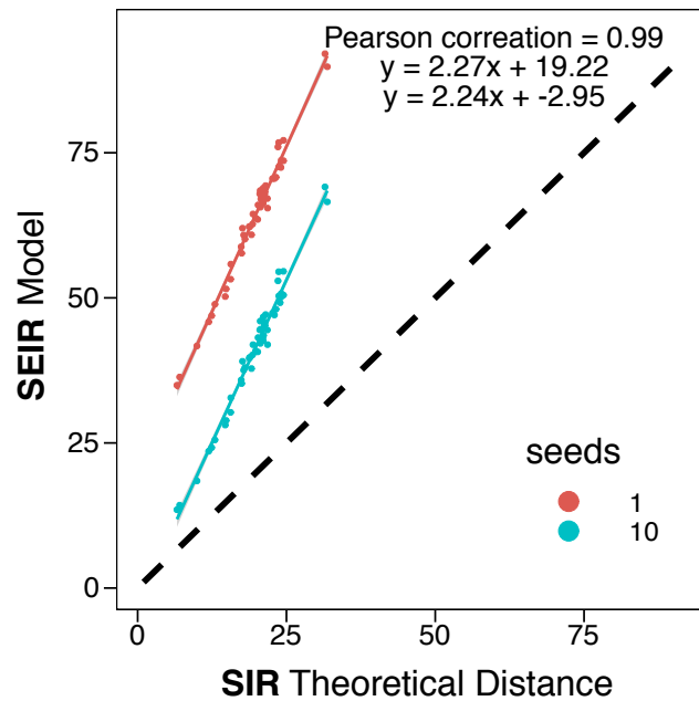
FIG. 3: Comparison between the hitting time obtained after 10^3 simulations of the SEIR model in our metapopulation scheme, with 1 or 10 seeds initially placed in the province of Barcelona, and the theoretical distance in a SIR metapopulation model.
