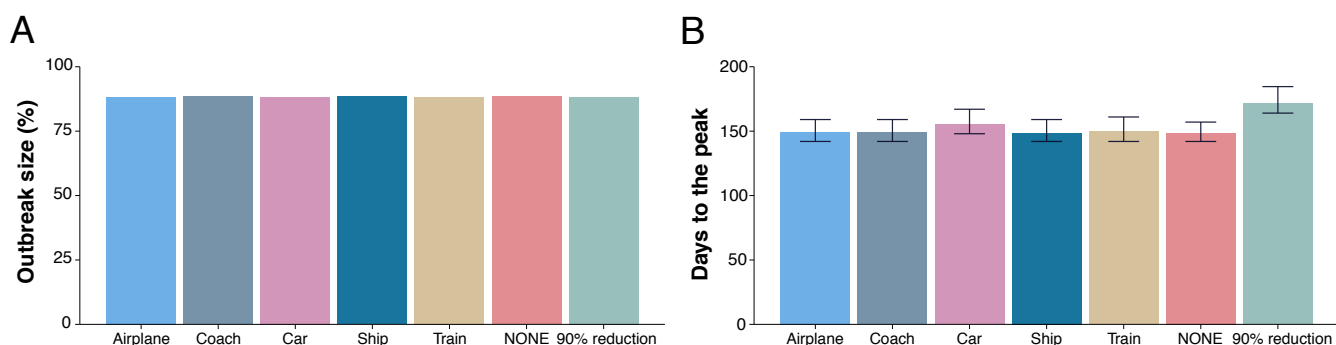
FIG. 6: Evaluating the impact of mobility reduction. Panel (A) shows the fraction of individuals who were affected by the disease by the end of the epidemic, whereas panel (B) displays the time from the arrival of the first infected individual to the country until the peak of the epidemic, i.e., the day with the maximum number of infected individuals. In all cases the epidemic starts with 10 infected individuals in the province of Barcelona.
