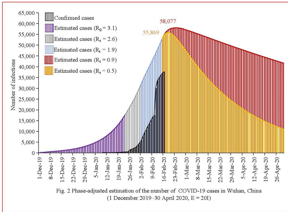
Fig. 2 Phase-adjusted estimation of the number of COVID-19 cases in Wuhan, China (1 December 2019–30 April 2020, E = 20I).
