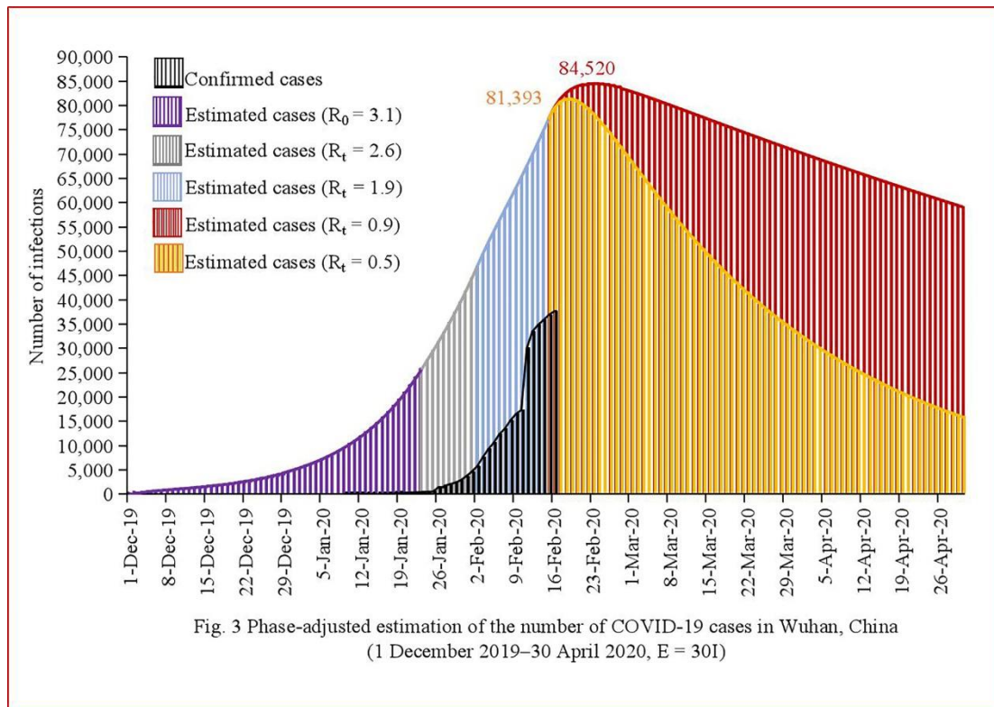
Fig. 3 Phase-adjusted estimation of the number of COVID-19 cases in Wuhan, China (1 December 2019–30 April 2020, E = 30I).
