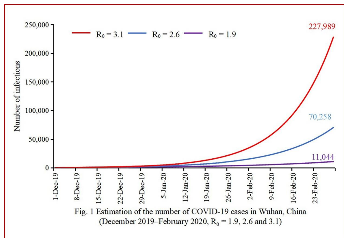
Fig. 1 Estimation of the number of COVID-19 cases in Wuhan, China (December 2019–February 2020, R_0 = 1.9, 2.6 and 3.1 ).
