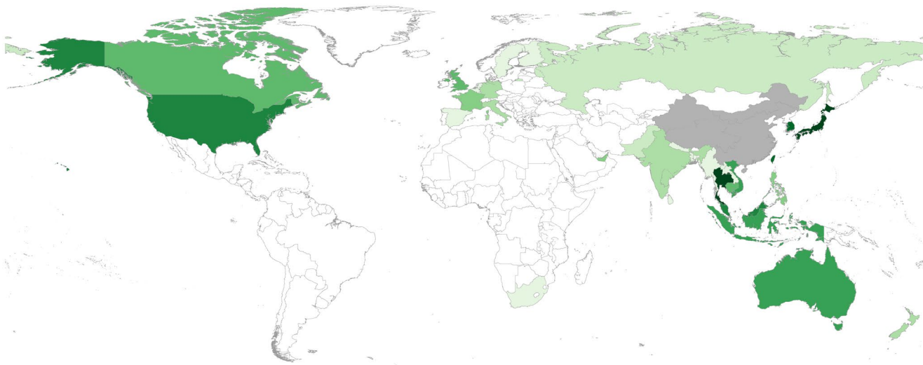
Estimated number of imported cases from Wuhan (Posterior Median)
