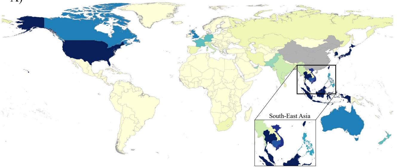
Local Outbreak Risk (Main Analysis)
