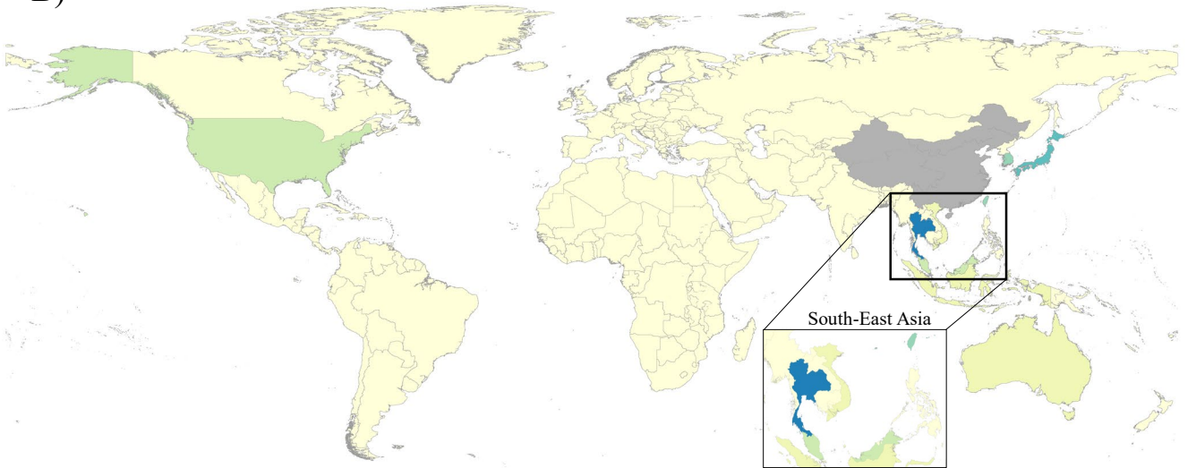
Local Outbreak Risk (95% Isolation)
