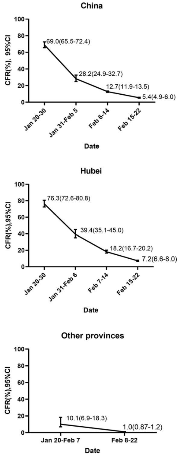
Fig. 3 Estimated CFR of COVID-19 during different time periods in China, Hubei and other provinces
