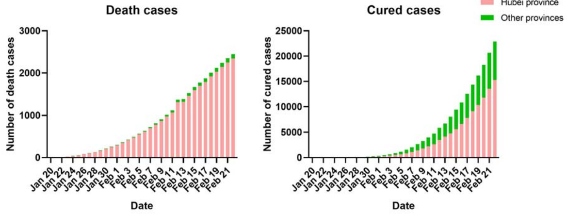
Fig.1 Cumulative numbers of death and cured cases in Hubei and other provinces
