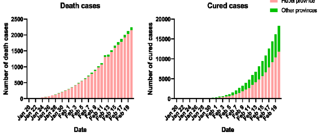
Fig.1 Cumulative numbers of death and cured cases in Hubei and other provinces
