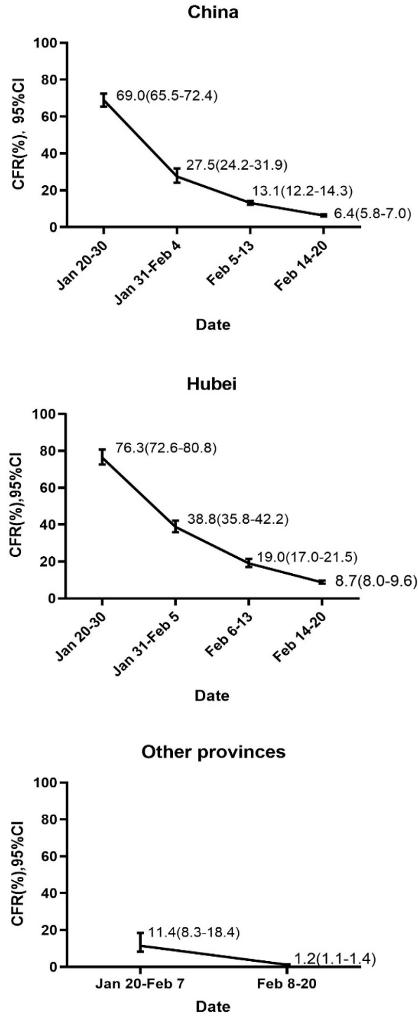
Fig. 3 Estimated CFR of COVID-19 during different time periods in China, Hubei and other provinces
