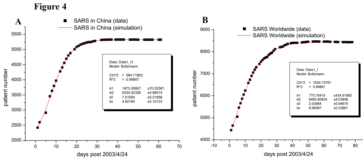
361 362 Figure 4. Fitting the cumulative number of confirmed cases for 2003 SARS in China and 363 worldwide to Boltzmann function 364 The cumulative number of confirmed cases of 2003 SARS in China (panel A) and worldwide (panel B) 365 are shown as black squares, and the simulation results from Boltzmann function are plotted as red short 366 lines and parameters of each established function are shown in inserts. 367 368
