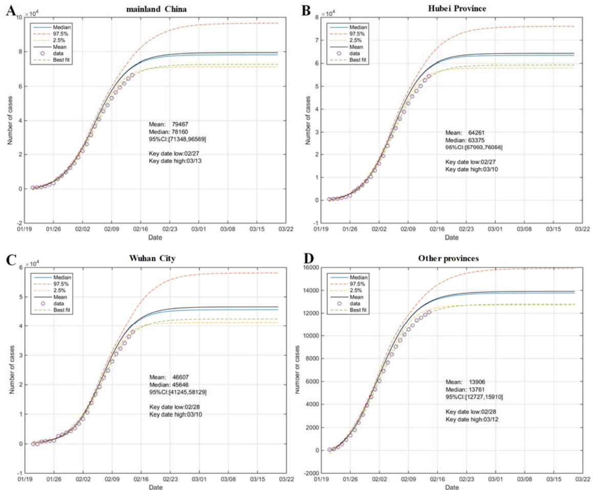
349 350 Figure 3. Analysis of the uncertainty of confirmed cases for mainland China, Hubei, other 351 provinces and Wuhan
