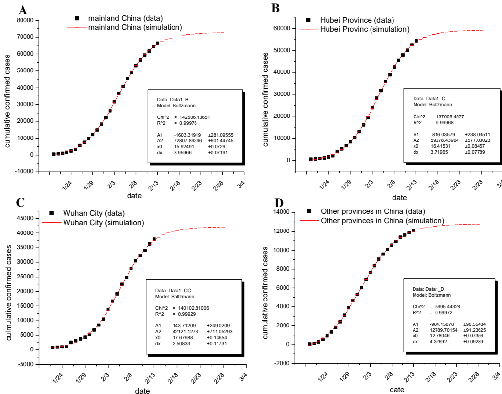
331 Figure 1. Fitting the cumulative number of confirmed cases from mainland China to 332 Boltzmann function
