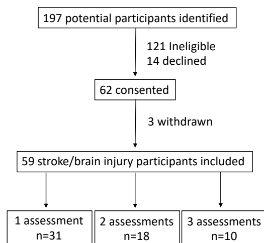
Fig. 1. Recruitment flowchart.
