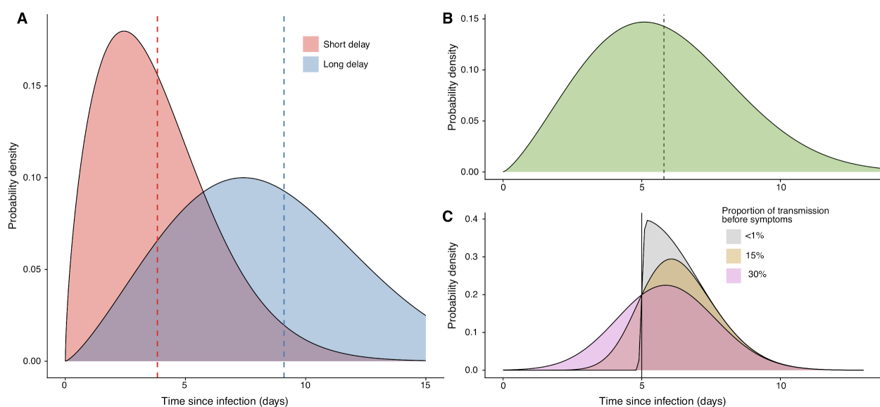
Figure 2: A) The short and long delay distributions between the onset of symptoms and isolation (mean marked by line). Parameter values and references are given in Table 1. B) The incubation distribution estimate fitted to data from the Wuhan outbreak by Backer et al. 24 . C) An example of the method used to sample the serial interval for a case that has an incubation period of 5 days. Each case has an incubation period drawn from the distribution in B, their serial interval is then drawn from a skewed normal distribution with the mean set to the incubation period of the case. In C, the incubation period was 5 days. The skew parameter of the skewed normal distribution controls the proportion of transmission that occurs before symptom onset, the three scenarios explored are <1% of transmission before onset (grey), 15% of transmission before onset (gold), and 30% of transmission before onset (pink).
