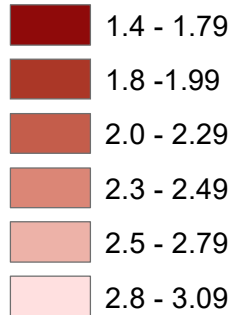
Harmonic mean of the arithmetic means of COVID-19 epidemic doubling times
