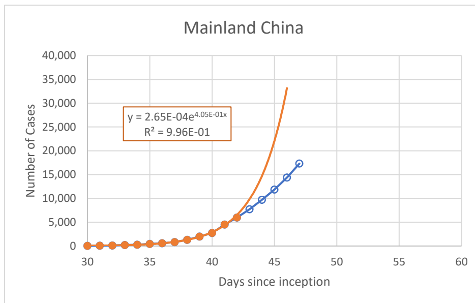
Figure 1 Evolution of recorded infection cases. Orange points (days 30 – 42) used to predict exponential growth. From day 42 there is a significant slowing of the infections.
