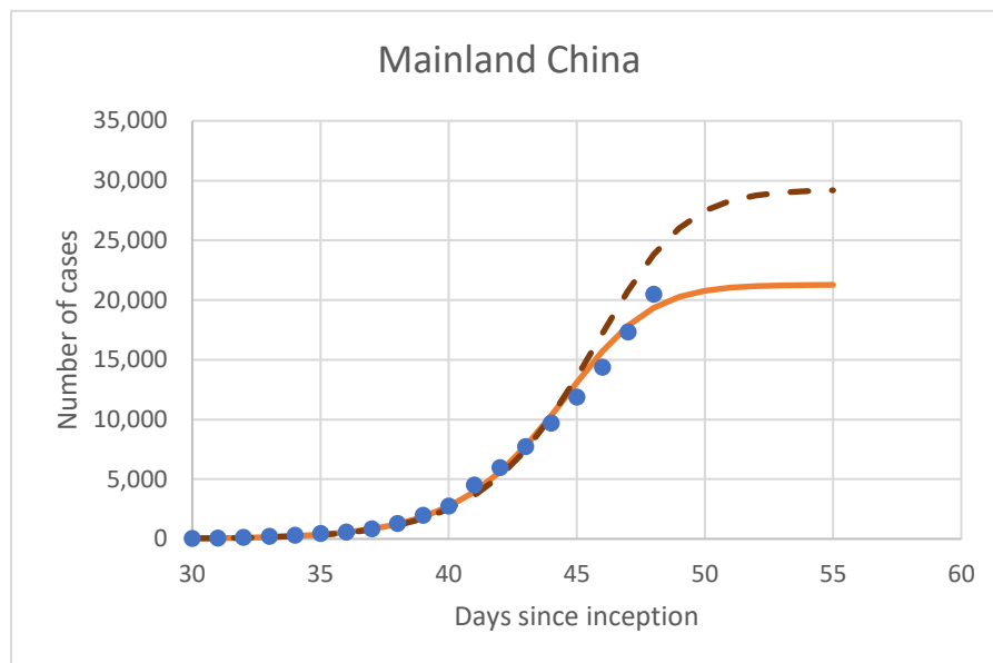
Figure 4 Recorded infection cases (up to day 48 = February 3). Orange line denote predictions from the initial 13-day dataset used for model calibration. Broken brown line shows model predictions using all data. Blue points fit model predictions.
