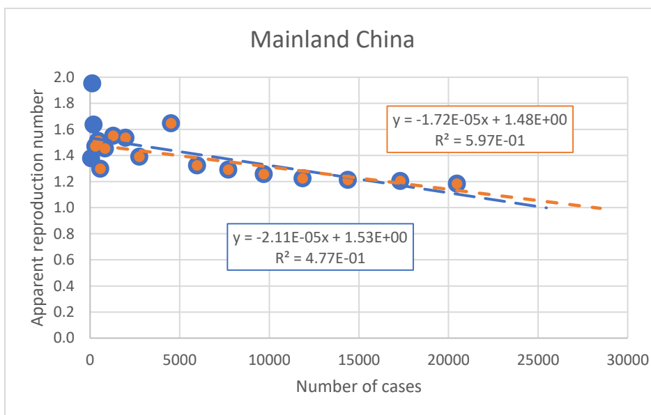
Figure 2 Linearization of the effective reproduction number with number of cases
