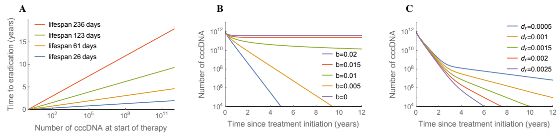
Fig 4. Effect of NA treatment predicted by the model. A: Predicted time for cccDNA to be eradicated in the absence of any cccDNA reproduction ( b=0 ). B: cccDNA dynamics whilst on treatment, assuming some residual reproduction. For all runs d=0.002 per day, \delta=0.006 per day, c=0 , q=0 . C: cccDNA dynamics on treatment, assuming no residual reproduction ( b=0 ) but 0.1% cccDNA is long-lived, for different death rates of long-lived cells, d_r per day. For normal cells d=0.002 , \delta=0.006 , c=0 , q=0 , and for long-lived cells \delta r=0 , c_r=0 , q=0 . The maximum number of cccDNA was assumed to be 10^{12} , and all model runs were started at equilibrium in the absence of treatment ( b=0.3 ).
