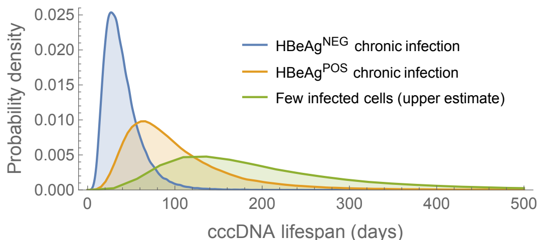
Fig 2. Probability distributions for cccDNA lifespan during different stages of HBV infection. The distributions for cccDNA in stable HBeAg POS and HBeAg NEG chronic infection are based on the neutral mutation rate and rate of neutral evolution (orange and blue lines, respectively). If the cccDNA burden during HBeAg NEG infection is not stable, but gradually falling (i.e. the basic reproduction number, R_0 , is less than one) the lifespan will be slightly less than inferred here. The upper estimate reflects the maximum likely cccDNA lifespan when few cells are infected, based on the neutral rate of evolution during HBeAg-positive infection and assuming no cccDNA survives mitosis ( q=0 ; green line).
