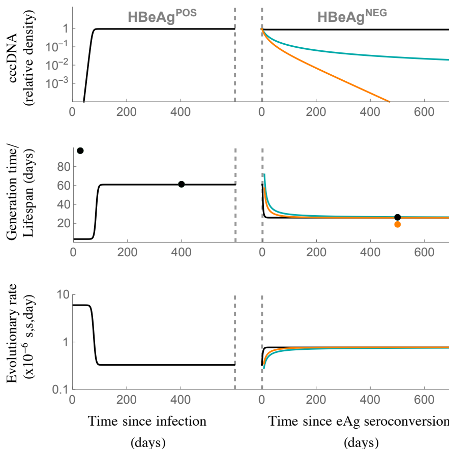
Fig 3. Population and evolutionary dynamics of cccDNA for the within-host model. We assumed no cccDNA survives mitosis ( q=0 ; see S1 Fig for the case where q=1 ). The model was parameterised assuming the generation time, g , during chronic HBeAg POS infection is 61 days, and during chronic HBeAg NEG infection is 26 days, in line with our predictions for cccDNA generation time in vivo . The top panel shows cccDNA burden, where 1 represents the maximum. The middle panel shows the viral generation time (lines) and cccDNA lifespan during key stages of infection (dots, derived from Eqs 9 and 10). The bottom row shows the evolutionary rates. Black line: replicative capacity during HBeAg NEG infection remains the same as during HBeAg-positive infection ( b_{eAg+} = b_{eAg-} = 0.3 per day). Blue line: replicative capacity falls to b_{eAg-} = 0.038 per day during HBeAg NEG infection, and R_0 = 1 . Orange line: replicative capacity falls to b_{eAg-} = 0.038 per day and R_0 = 0.7 . See Table 1 for all other parameters.
