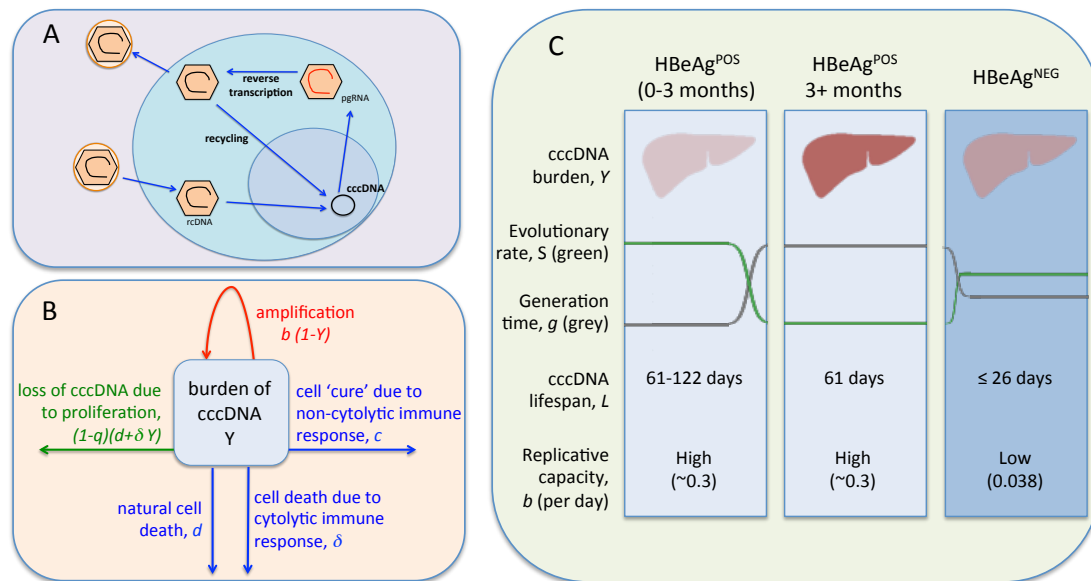
Fig 1: Summary of the HBV life cycle, mathematical model, and estimated cccDNA lifespan.
