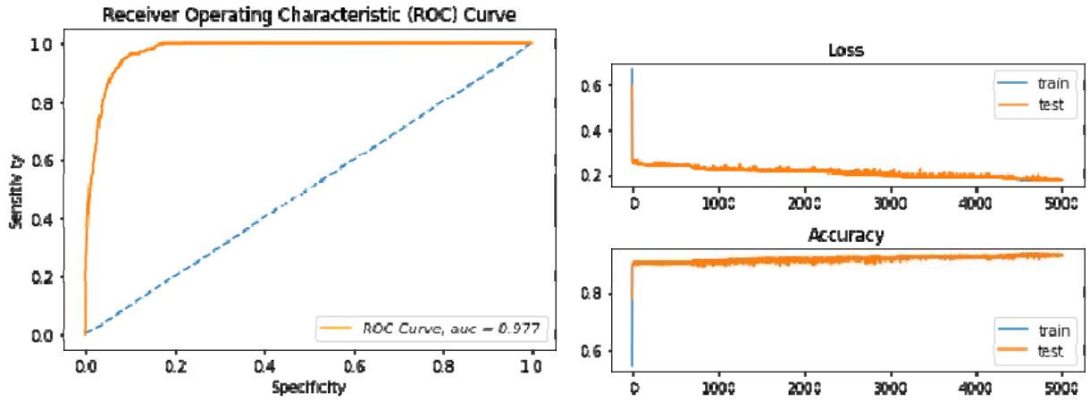
Figure 1. Receiver -Operator Curve for FLAIM-DNN-4RS and the loss and accuracy curve during training
