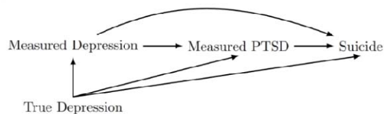
DAG A: measurement error for depression
