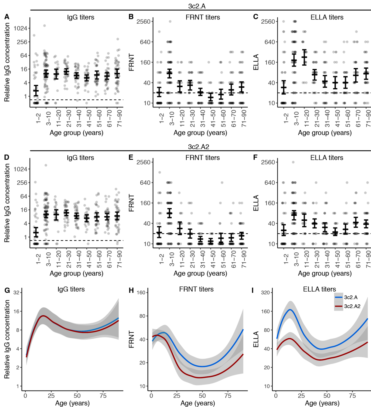
497 498 Figure 1. Antibody titers to contemporary A(H3N2) viruses in serum collected prior to the 2017-2018 499 season. ELISAs were completed to quantify the levels of 3c2.A (A) and 3c2.A2 (D) HA-specific IgG 500 in serum from different aged humans. FRNTs were completed to quantify the levels of 3c2.A (B) and 3c2.A2 501 (E) neutralizing antibodies in serum from different aged humans. ELLAs were completed with viruses that 502 had 3c2.A NA (C) and 3c2.A2 NA (F) to quantify NA-specific inhibitory antibodies in serum from different 503 aged humans. For A-F, the geometric mean titers are shown as cross bars and 95% confidence intervals 504 as error bars. (G-H) Data from panels A-F are summarized. Lines (blue=3c2.A; red=3c2.A2) are Loess 505 curves showing smoothed geometric mean titers with the 95% confidence intervals shaded. Dashed lines 506 in panels A-F represent the limit of detection for each assay. 507
