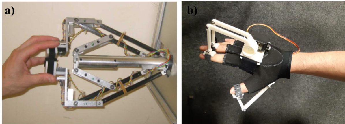
341 Figure 3. Robotic hand rehabilitation devices: a) An end-effector device (Haptic Knob) 342 used in one of the extracted studies [60,98], b) a wearable hand exoskeleton/orthosis 343
