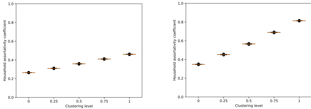
(a) Household assortativity coefficient as calculated over the entire population for clustering levels 0, 0.25, 0.5, 0.75 and 1.
