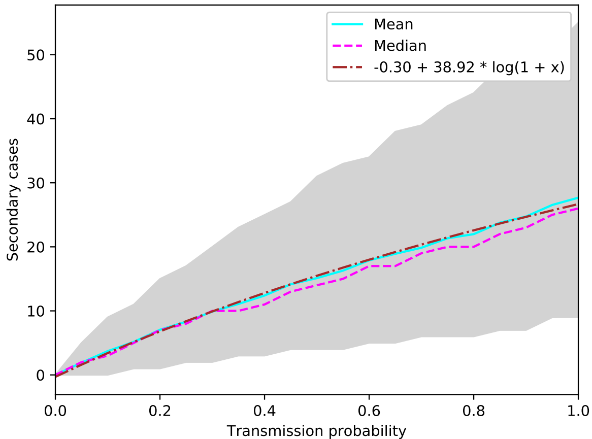
Figure 1. Mean (solid blue line), median (dotted pink line) and 95% percentile interval (grey shape) of secondary cases caused by an index case over 1,000 simulations per value for P_{\text{transmission}} . The dotted brown line represents the function we fit to the data.
