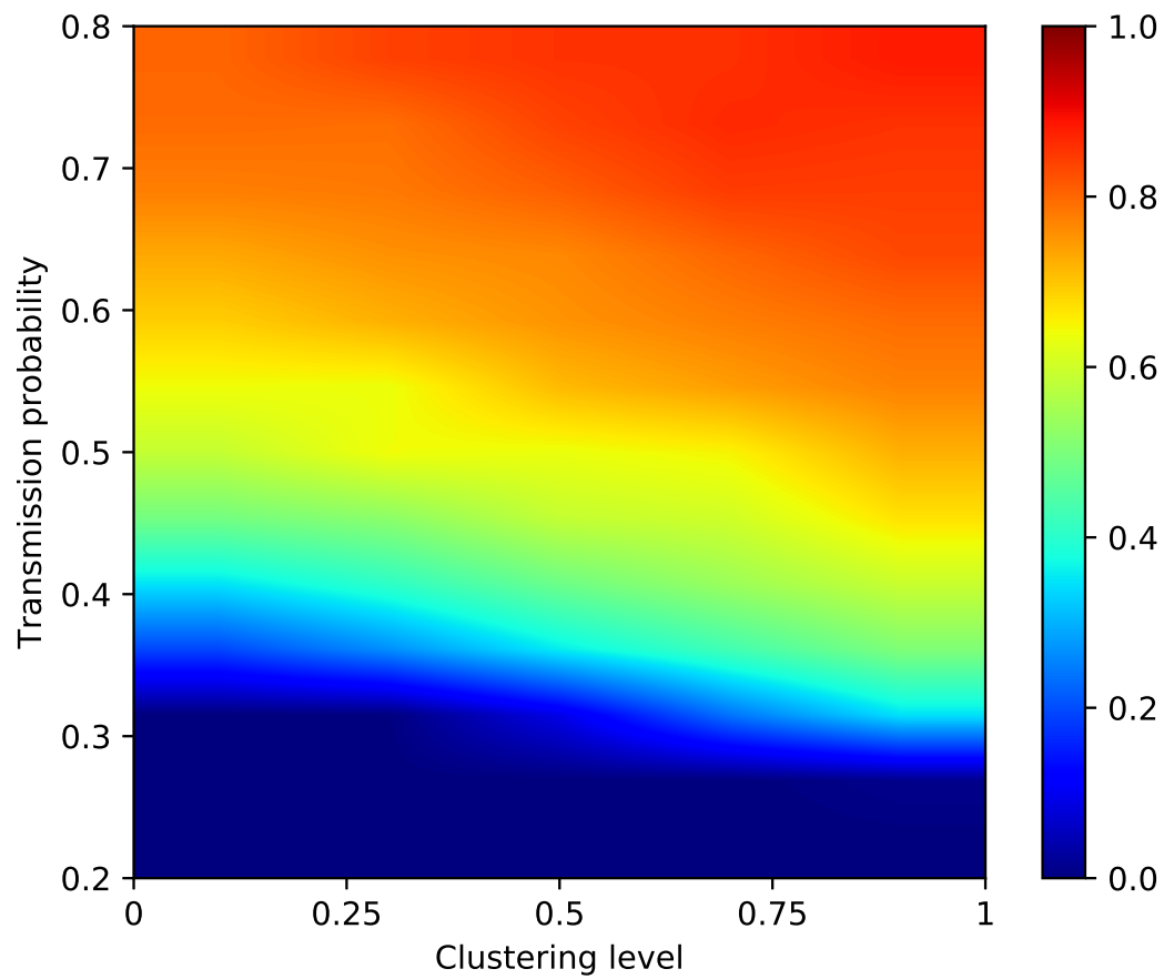
Figure 5. Fraction of persistent outbreaks for clustering levels 0, 0.25, 0.5, 0.75, and 1, with values for P_{\text{transmission}} ranging from 0.2 to 0.8. Per scenario, we ran 1,000 simulations. Extinction threshold = 5,000 cases.
