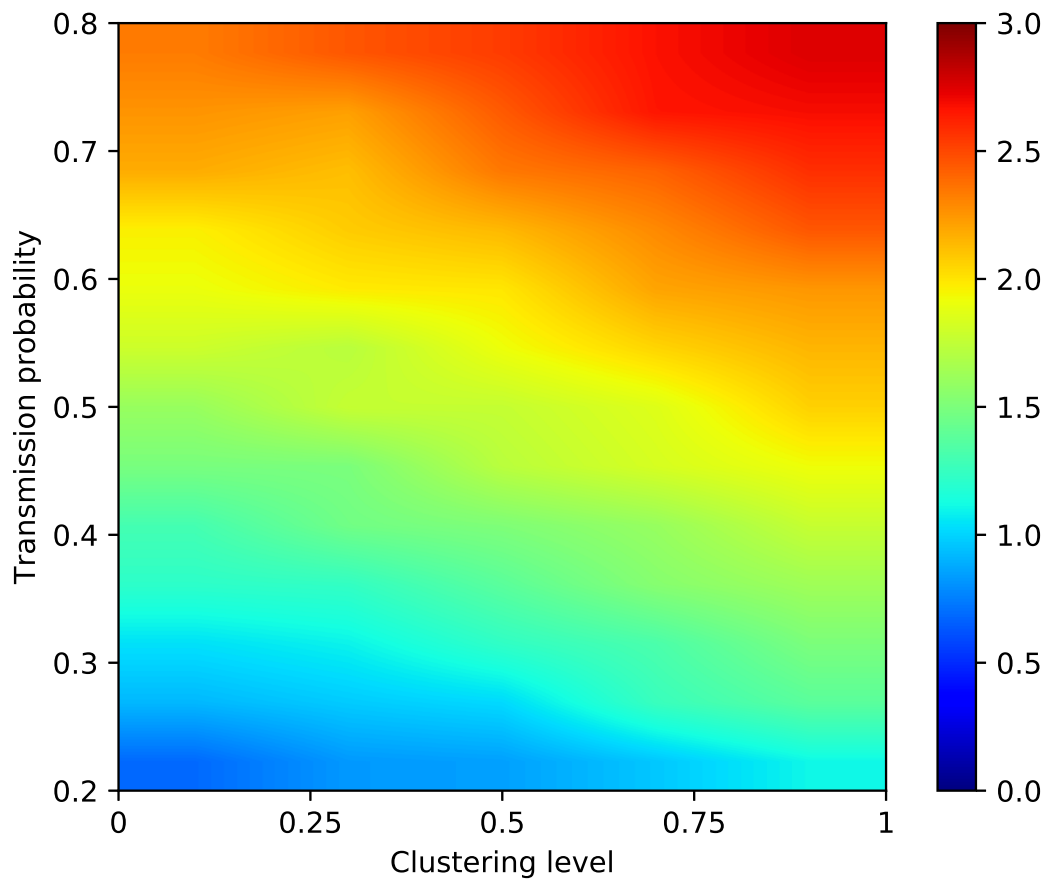
Figure 4. Effective R for clustering levels 0, 0.25, 0.5, 0.75 and 1 and values of P_{\text{transmission}} from 0.2 to 0.8 ( R_0 \sim 6.80 to 22.58). Results are based on 1,000 simulations per scenario.
