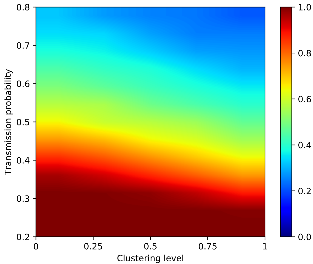
Figure 6. Mean escape probability for clustering levels 0, 0.25, 0.5, 0.75, and 1, with P_{\text{transmission}} ranging from 0.2 to 0.8. We calculated the average escape probability over 1,000 runs for each scenario.
