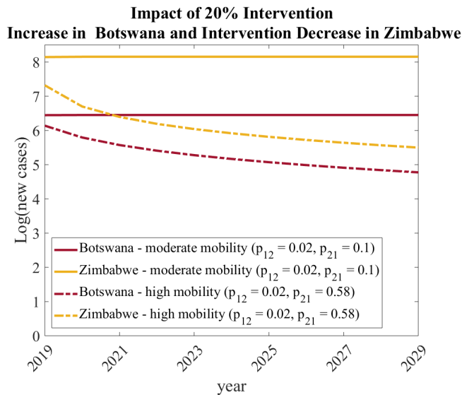
Fig. 13: Impact of a Worsening of Malaria Conditions in Zimbabwe and Interventions in Botswana on New Cases. The total number of new malaria cases (Equations (7)) and (8)) under the scenario that Botswana increases \mu_1 by 20 percent and Zimbabwe increases a_2 by 20 percent under two mobility strategies: moderate (solid curves, system R_0 = 1.941 ) and high (dotted curves, system R_0 = 0.994 ).
