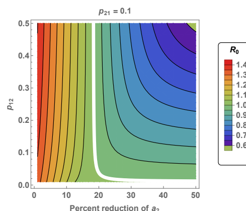
Fig. 9: System Level R_0 Under Intervention in Zimbabwe. Impact on the system total R_0 (Equation (6)) by varying visitation rate from Botswana to Zimbabwe and decreasing the human biting rate of the mosquitoes in Zimbabwe ( a_2 ), corresponding to improvement in the insecticide-treated bednet coverage.
