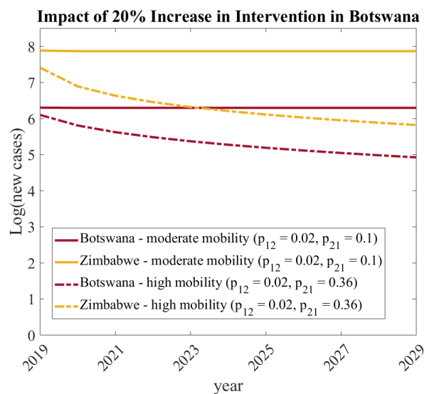
Fig. 8: Impact of Mobility and Successful Intervention in Botswana on New Cases. The total number of new malaria cases (Equations (7) and (8)) under the scenario that Botswana increases \mu_1 by 20 percent under two mobility strategies: high (dotted curves, Total R_0 = 0.995 ) and moderate (solid curves, Total R_0 = 1.35 ).
