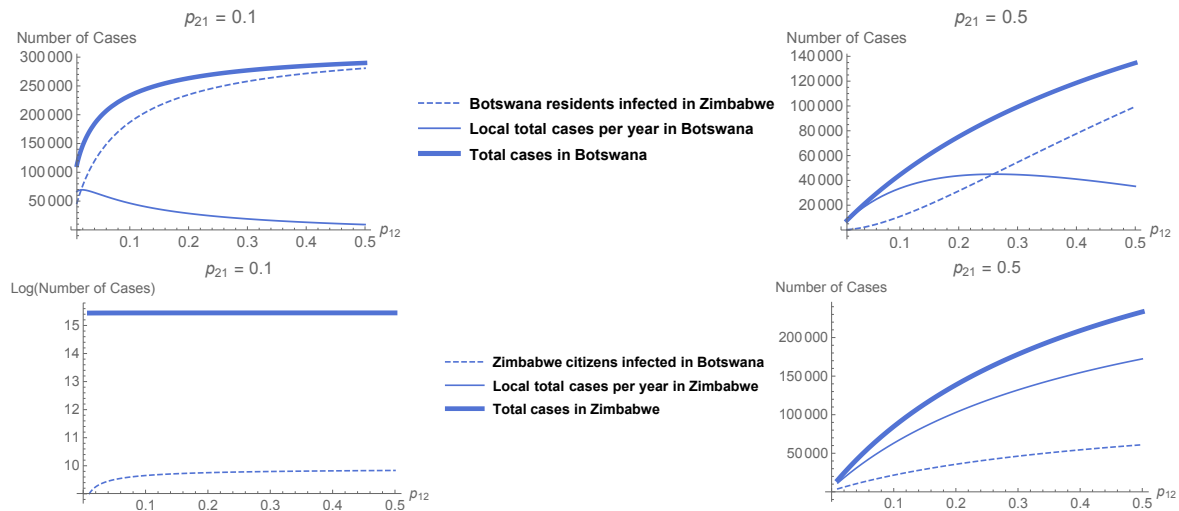
Fig. 6: Impact of Mobility on Local and Imported Malaria Cases. We fix the visitation rate of Zimbabwe residents visiting Botswana ( p_{21} ) at a low (Left) and high (Right) rate and then vary the visitation rate of Botswana residents to Zimbabwe on the x-axis ( p_{12} ). We plot the steady-state number of infections per year corresponding to the number of residents infected in Botswana (Top) and Zimbabwe (Bottom). For both countries, there are substantially fewer cases under high rates of visitation from people in Zimbabwe to Botswana. Left: As visitation to Zimbabwe increases, the number of total cases in Botswana increases but the number of locally acquired cases decreases. The number of cases in Zimbabwe is only modestly impacted. Right: As visitation to Zimbabwe p_{12} increases, the locally acquired cases in Botswana decrease by approximately 80%. With higher visitation rates from Zimbabwe to Botswana ( p_{21} = 0.5 ) we have roughly half of the total cases we obtain annually in Botswana with lower levels of visitation.
