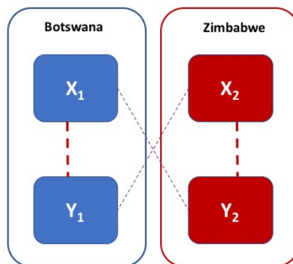
Fig. 3: Conceptual Two-Patch Malaria Model. Patch 1 (Botswana) and Patch 2 (Zimbabwe) contain both infected humans ( X_1 and X_2 ) and infected mosquitoes ( Y_1 and Y_2 ). Interactions that could result in infection are identified with dotted lines. Thick red dotted lines denote within patch routes of infection, while the thin purple dotted lines denotes infection acquired by human mobility.
