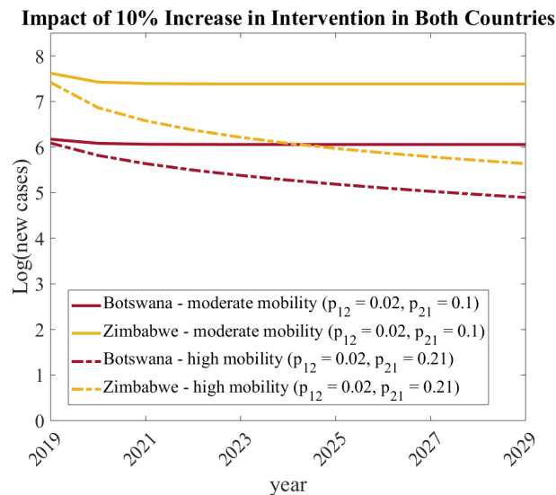
Fig. 12: Synergistic Impact of Improved Interventions in Both Countries. The total number of new malaria cases (Equations (7) and (8)) under the scenario that Botswana increases \mu_1 by 10 percent and Zimbabwe decreases a_2 by 10 percent under two mobility strategies: moderate (solid curves, system R_0 = 1.1 ) and high (dotted curves, system R_0 = 0.994 ).
