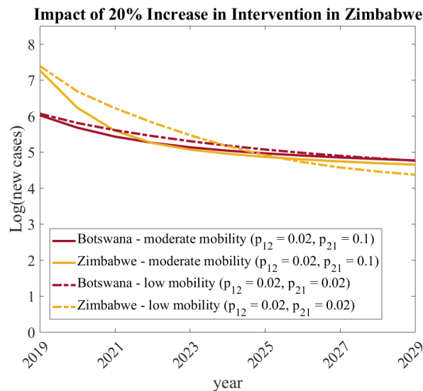
Fig. 10: Impact of Mobility and Successful Intervention in Zimbabwe. The total number of new malaria cases (Equations (7) and (8)) under the scenario that Zimbabwe decreases a_2 by 20 percent under two mobility strategies: moderate (solid curves, system R_0 = 1.005 ) and low (dotted curves, system R_0 = 0.998 ).
