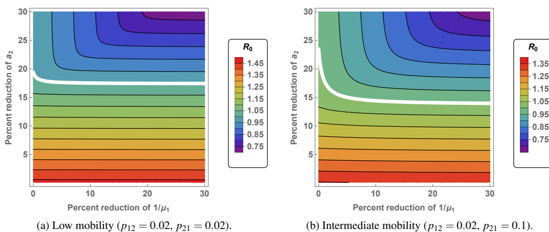
Fig. 11: System Level R_0 Under Intervention in Both Countries. (a) We show percent reduction of \frac{1}{\mu_1} in Botswana on the x-axis, corresponding to decreasing the lifespan of a mosquito with successful usage of IRS (spraying) and percent reduction of a_2 in Zimbabwe (on the y-axis), corresponding to the decreasing of mosquito feeding rate through ITN intervention, under the scenario of low mobility. (b) This is the same as part (a), but for the scenario of intermediate mobility.
