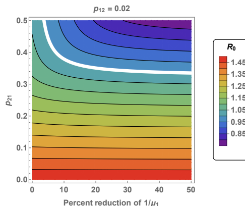
Fig. 7: System Level R_0 Under Intervention in Botswana. We fix p_{12} (the rate of visitation from Botswana to Zimbabwe) and p_{21} (the rate of visitation from of Zimbabwe to Botswana) and vary 1/\mu_1 , parameter controlling the mosquito death rate (mosquito lifespan in days), and reflecting changes in the insecticide spraying intervention in Botswana. The system total R_0 (Equation (6)) can be reduced below 1 by decreasing 1/\mu_1 , but for larger values of 1/\mu_1 the R_0 is dominated by p_{21} .
