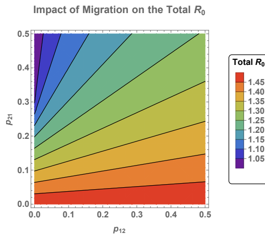
Fig. 4: System Level R_0 Under Varying Mobility. While Botswana and Zimbabwe are both sources with reproduction numbers R_0 = 1.01 and R_0 = 1.5 , respectively, the system level R_0 cannot be driven below 1 with mobility alone.
