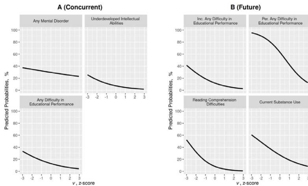
Figure 2: Static prediction of concurrent and future mental health, substance use and educational outcomes
