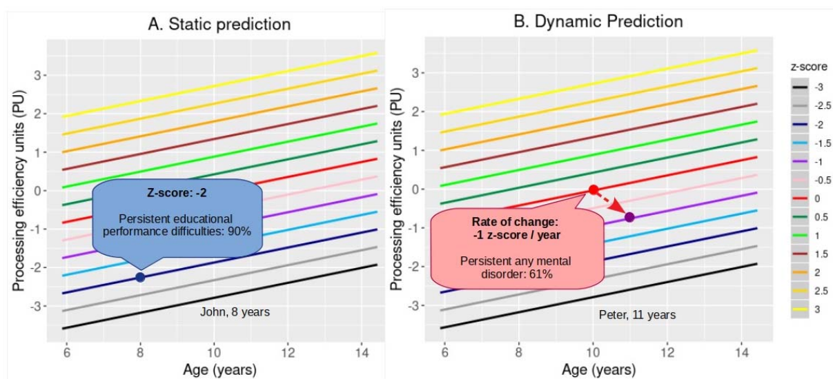
Figure 4: Cognitive development chart examples
