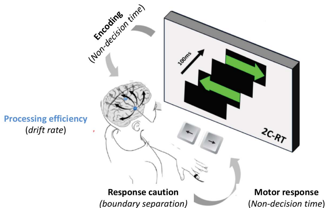
Figure 1: EZ-diffusional model components
