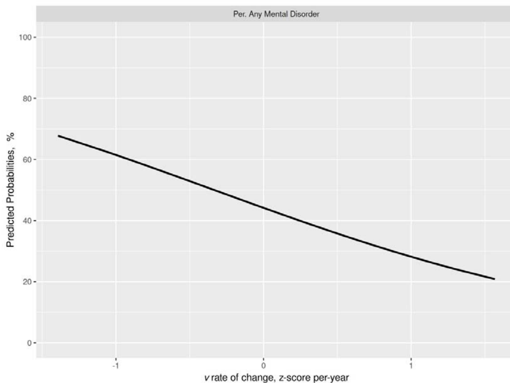
Figure 3: Dynamic prediction of future mental health problems
