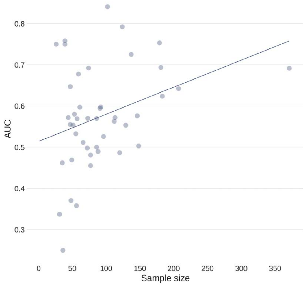
Figure 2. Scatterplot illustrating relationship between number of participants and classification performance across sites.
