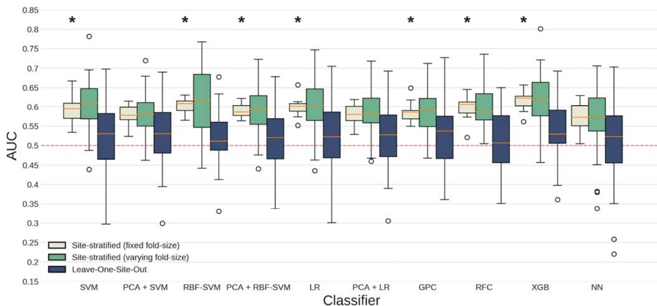
Figure 1. Performance for multi-site classification using different algorithms and cross-validation schemes. Boxplots summarize AUC scores obtained across CV-iterations; the dashed line represents chance-level performance and asterisks indicate scores significantly different from chance (Mann-Whitney-U statistic; p < 0.05 Bonferonni corrected (10 classifiers x 3 CV types), see eSupplement for details). SVM=Support Vector Machine, PCA=Principal Component Analysis, RBF=Radial Basis Function, LR=Logistic Regression, GPC=Gaussian Processes Classification, RFC=Random Forest Classifier, XGB=XGBoost, NN=Neural Network.
